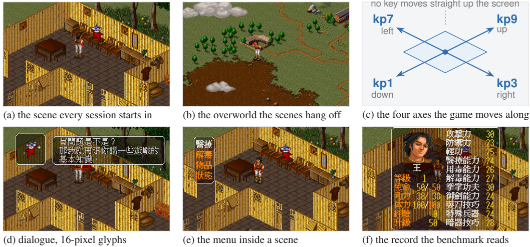
Figure 1: The environment at the resolution the model receives it, upscaled three times without interpolation. The two tiers of the world (a, b), the four axes along which the four movement keys move the character (c), and the three kinds of text panel through which every objective, choice and statistic is stated (d–f).
