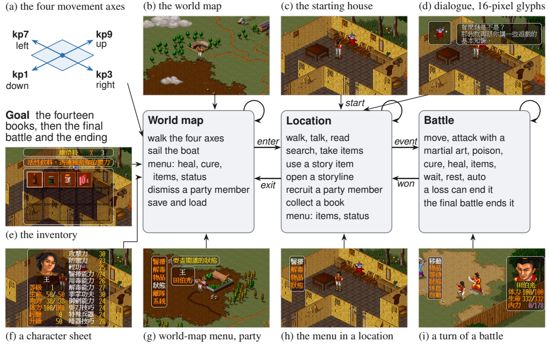
Figure 1: The game as a state chart of three states, each repeating the steps it lists, with the transitions between them. Every frame is one the model receives, upscaled three times without interpolation, and points at the state it shows.
