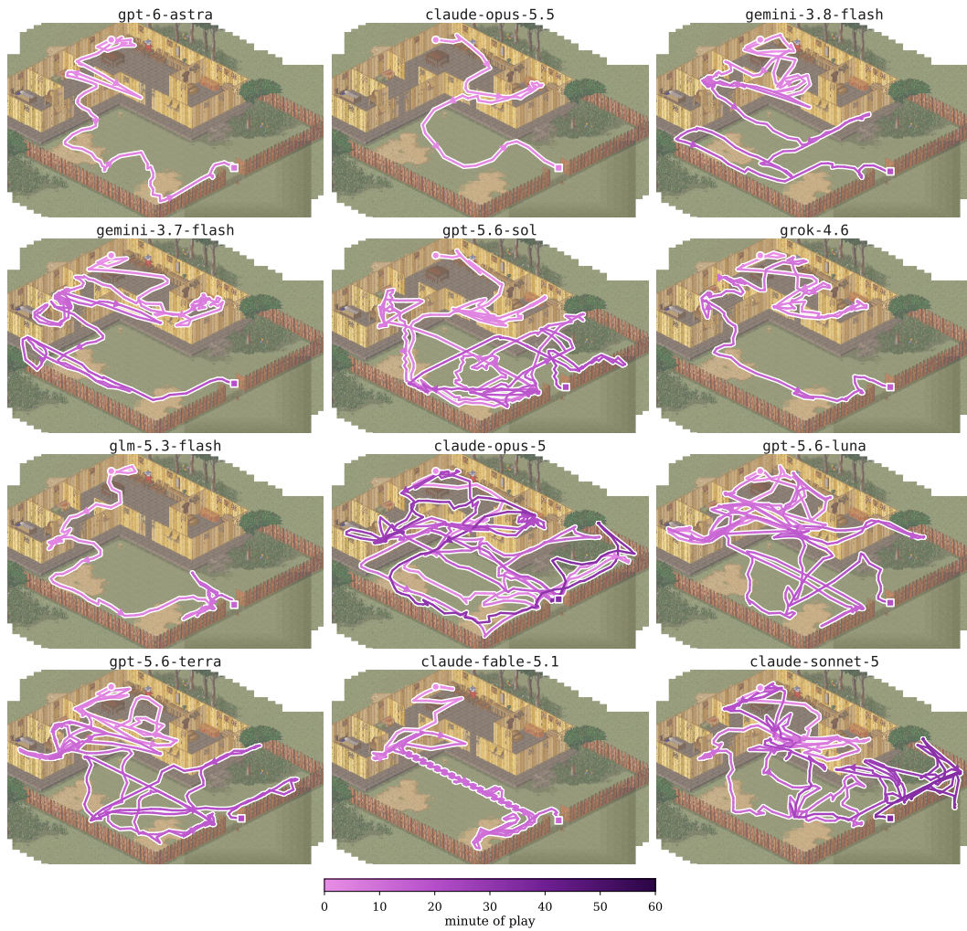
Figure 4: The walk of every model through the starting house in its session with the most milestones, from the spawn tile (circle) to the crossing (square). The colour gives the minute of play, on the scale shared with Figure 5, and the arrowheads the direction. The panels follow the upper panel of Figure 3, and Appendix D describes how a walk is read.
