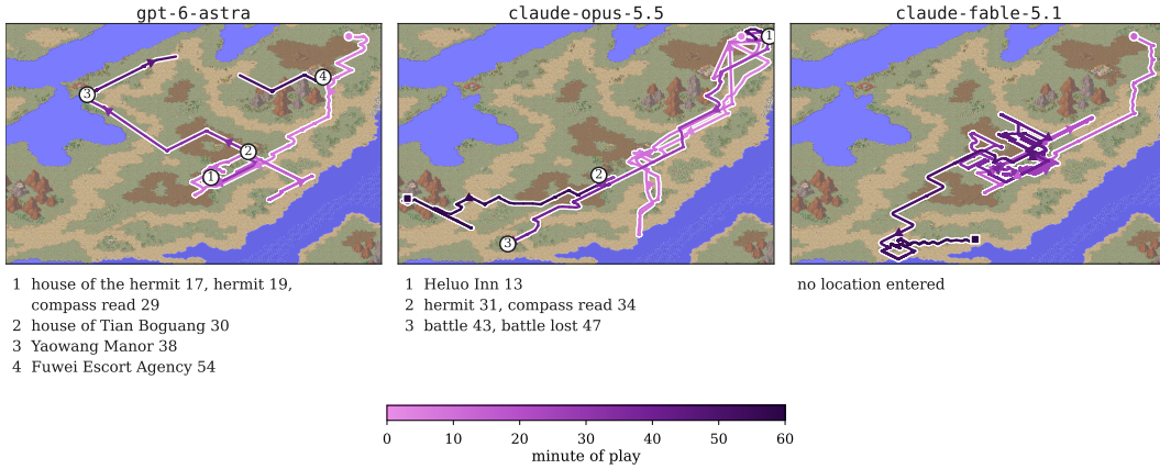
Figure 5: Three walks on the world map in the first hour, coloured by the minute of play: the session of gpt-6-astra that entered the most locations, the session of claude-opus-5.5 with the most milestones, and the session of claude-fable-5.1 that stayed longest on the world map without entering a location. A numbered marker stands at the last point on the world map before a location entered or a panel read from the replay, and the list under each panel gives its markers with their minutes. A gap in a path is a visit to a location or a loaded save.
