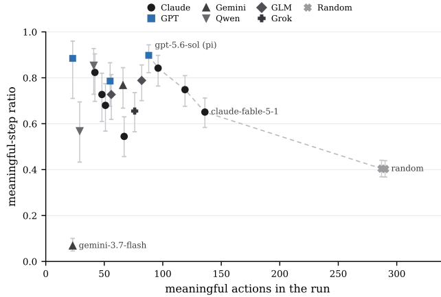
Figure 6: Quality against throughput, with 95% Wilson intervals on the ratio. Neither axis alone is a score: the ratio rewards near-inaction and the count rewards speed alone. The dashed line joins the runs dominated on neither axis.
