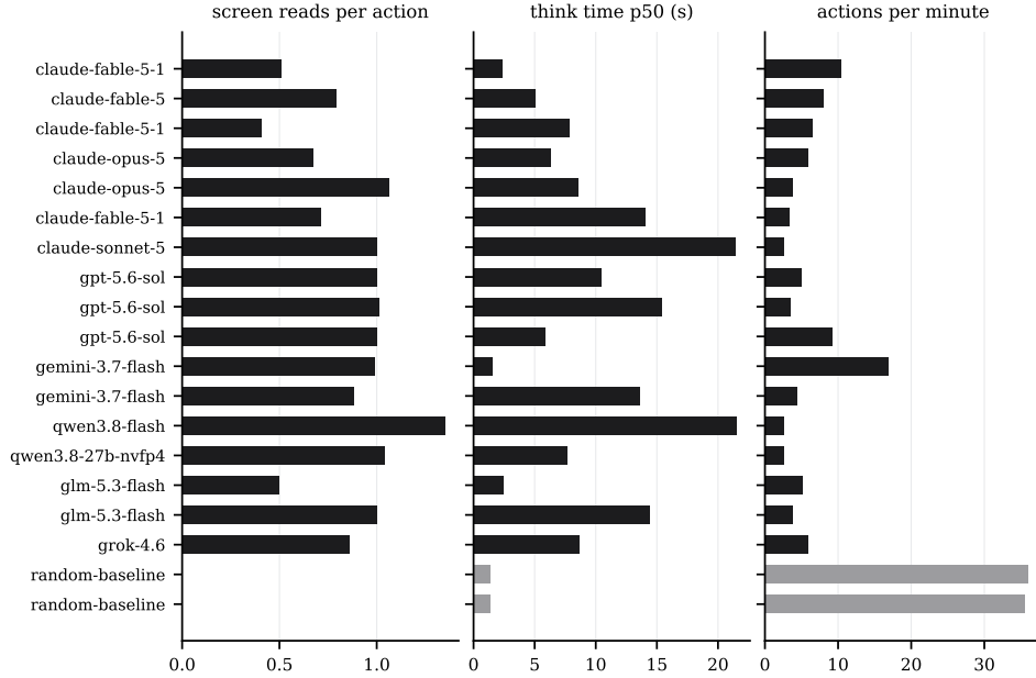
Figure 7: Behavioural signatures, one row per scored session: screen reads per action, median think time in seconds, and actions per minute. The random baseline is the pair of grey rows.
