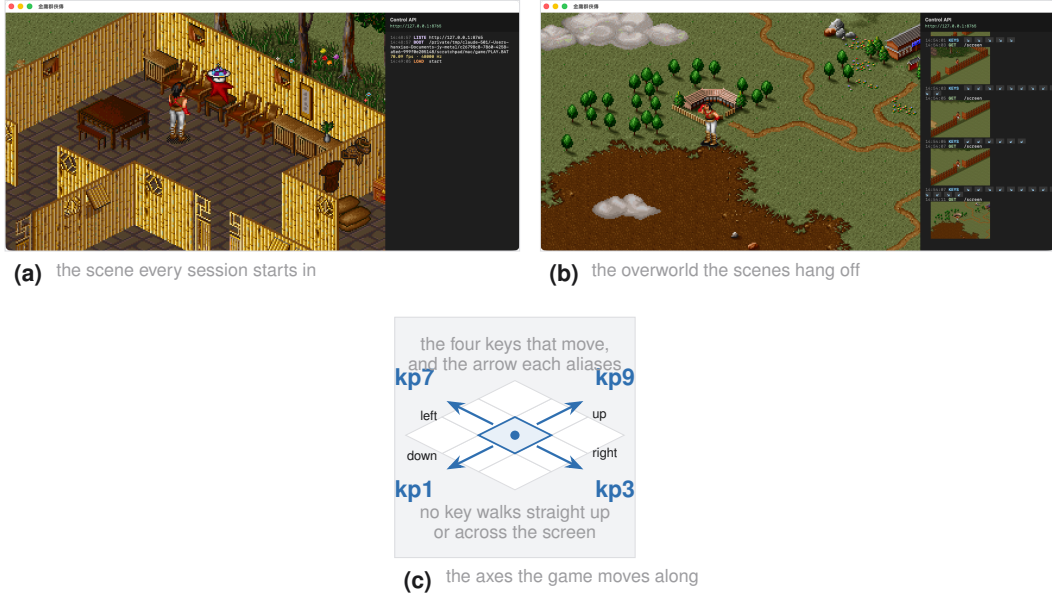
Figure 1: The native runner on the two tiers of the world, and the geometry that connects them to the keyboard. The right pane of the window logs every control call with the key it sent and the frame it returned; a session sees only the frame.
