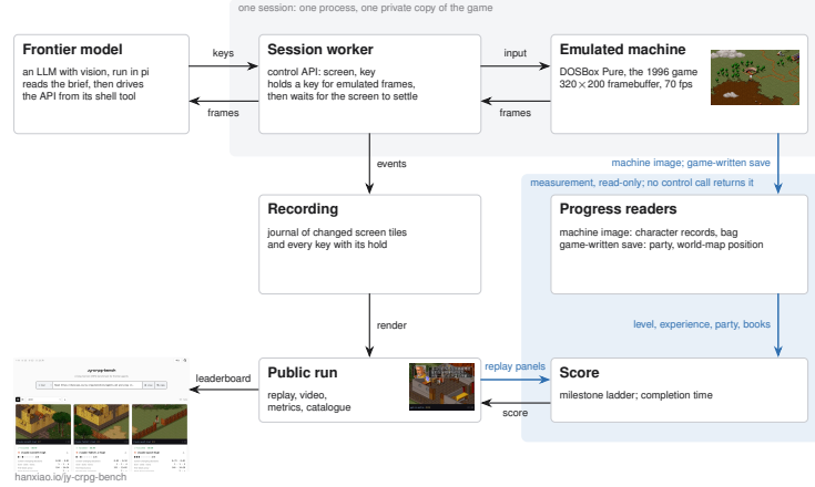
Figure 5: A frontier model, hosted in pi, drives the control API of its own session; the recording feeds the public replay, and progress is read from the emulated machine, from the save the game writes and from the replay, through paths the control API does not expose.
