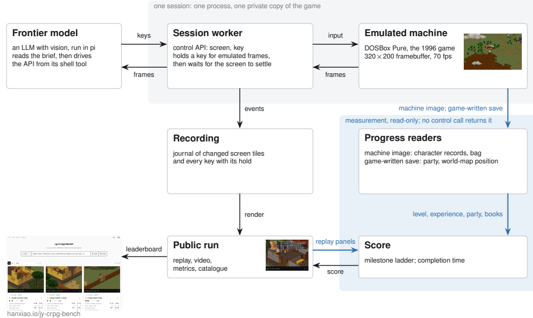
Figure 2: A frontier model, hosted in pi, drives the control API of its own session; the recording feeds the public replay, and progress is read from the emulated machine, from the save the game writes and from the replay, through paths the control API does not expose.
