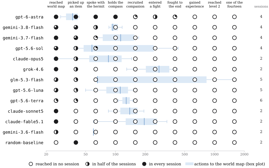
Figure 3: Milestones per model, ordered by milestones reached, then by the shares from the deepest milestone down, then by median actions to the world map. Each marker shows the share of sessions in which the model reached the milestone, and the number of sessions is given at the right. The box plot behind each row shows the actions taken to reach the world map across the sessions that crossed, on a log scale, with the box spanning the quartiles, the line inside it the median, and the thin line the range. The evidence for each milestone, and the record it comes from, is: a save written on the world map, or the world-map fingerprint (save, frame); an item count above the starting count, or the pickup message on screen (memory, replay); the portrait of the hermit (replay); the compass in the bag or on the item screen (memory, replay); a party of more than one, or a yes to the join prompt (save, replay); the card of the acting character (replay); the defeat banner or experience gained (replay, memory); experience above zero and a level above one (memory); a book in the bag or carried by the protagonist (memory). A session with no fight on its replay is counted as having gained no experience and no book, since both require a won fight.
