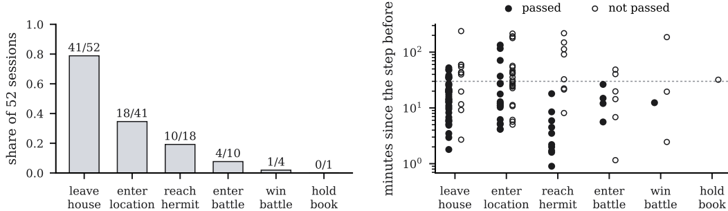
Figure 7: All model sessions through the steps a playthrough passes in order. Left, the sessions that passed each step, of those that passed the step before. Right, for each of those, the minutes from the step before to passing it (filled) or to its last key (open); the dashed line marks 30 minutes.
