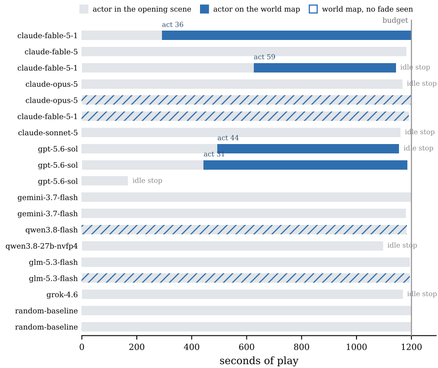
Figure 5: One row per scored session. Grey is time inside the opening scene and blue is time on the world map, with the action count at which the transition happened; hatched rows latched the map signature without a corroborating fade. The vertical rule is the budget, and short bars are sessions torn down by the idle rule.
