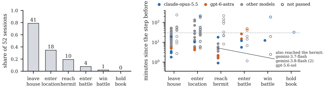
Figure 7: All model sessions through the steps a playthrough passes in order. Left, the sessions that passed each step. Right, the minutes from the step before to passing it (filled) or to the last key of a session that did not pass it (open), coloured by model; the dashed line marks 30 minutes.
