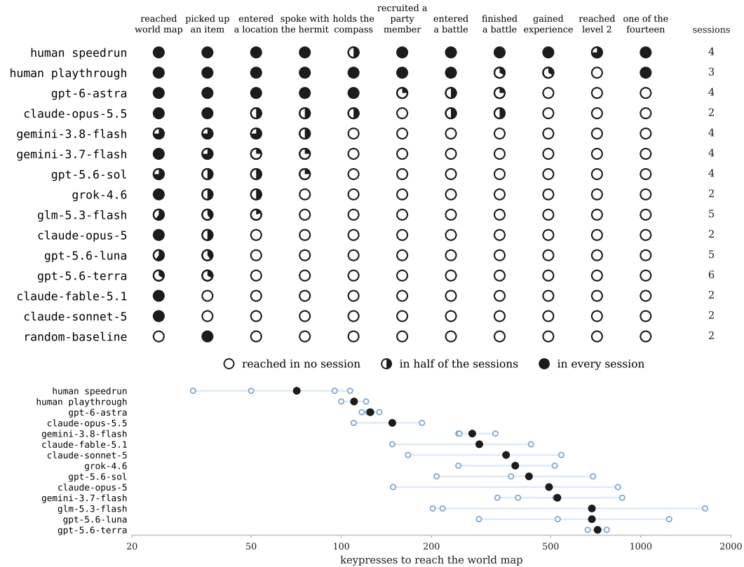
Figure 3: Milestones per model. The rows of the upper panel are ordered by the milestones reached and the rows of the lower panel by the mean keypresses to the world map, with the random baseline last. In the upper panel each marker shows the share of sessions in which the model reached the milestone, with the number of sessions at the right. The lower panel shows the keypresses to the world map across the sessions that crossed, on a log scale, with a light dot per session and a black dot for their mean. The two human rows are read from published videos, and Appendix D gives the record behind each milestone.
