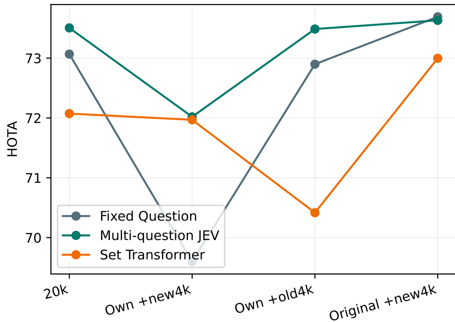
20k baseline and 24k equal-extra-budget controls
