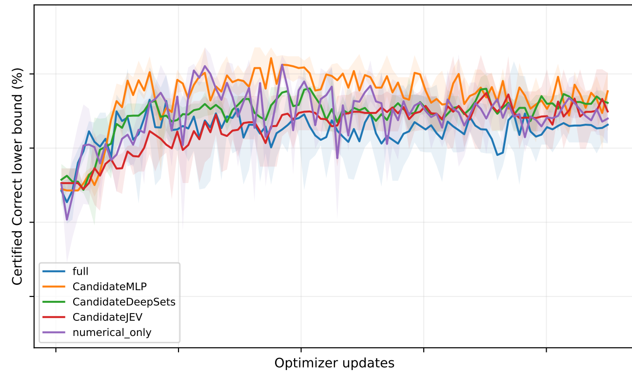
Phase XII frozen native v3 development validation: mean and range of 3 seeds Partial labels; UNKNOWN is not a negative. Best checkpoint chosen by known NLL + executed ranking loss.
