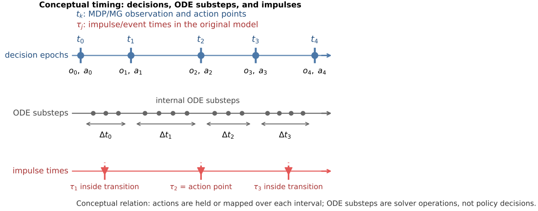
Figure 4: Conceptual relation among policy epochs, ODE substeps, and original-model impulse times. The checked learning environment uses fixed decision intervals, applies an isolation reset only at a decision epoch, and then integrates with fixed internal substeps. An impulse time \tau_j between epochs describes the broader continuous-time model; it is not an extra action taken by the current policy implementation.
