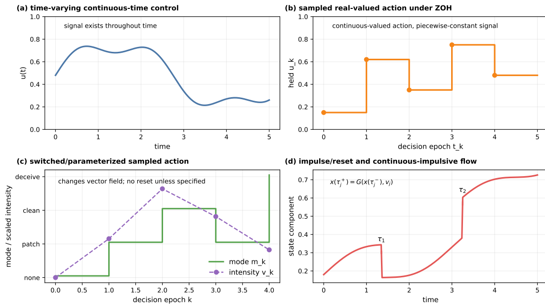
Figure 3: Control-action taxonomy used in this note. A continuous-time control is a time signal u(t) . A sampled real action u_k under zero-order hold is piecewise constant. A mode or parameterized action selects the interval vector field without a reset unless a jump map is specified. An impulse is defined by the reset x(\tau_j^+) = G(x(\tau_j^-), v_j) .
