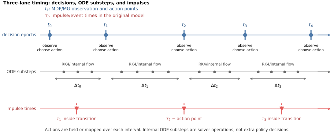
Figure 4: Three-lane action timing used in the sampled-data learning code. Decision epochs t_k are the points where the MDP or Markov game observes the state and chooses actions. ODE substeps are internal numerical integration steps. Impulse times \tau_j belong to the original continuous-time or impulse model and may coincide with, or fall between, decision epochs.
