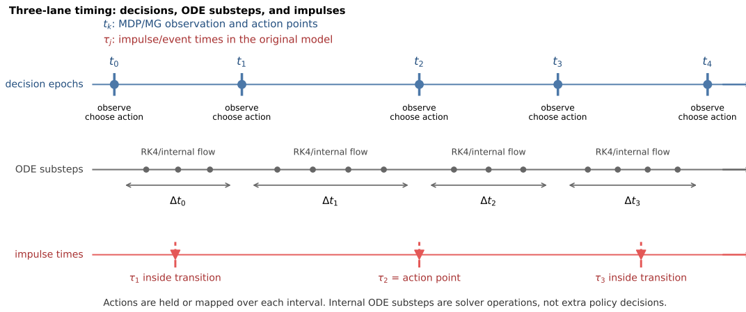
Figure 2: Three-lane action timing used in the sampled-data learning code. Decision epochs t_k are the points where the MDP or Markov game observes the state and chooses actions. ODE substeps are internal numerical integration steps. Impulse times \tau_j belong to the original continuous-time or impulse model and may coincide with, or fall between, decision epochs.
