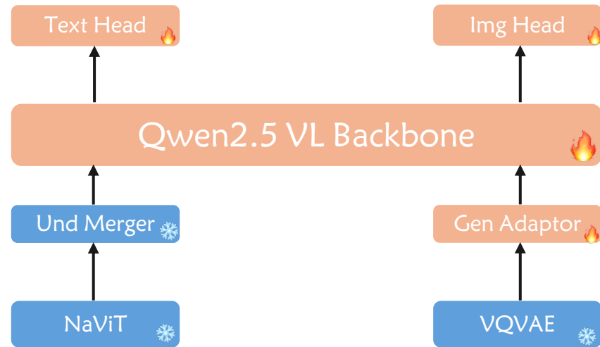
Stage 2: Understanding and Generation Joint Pretraining
