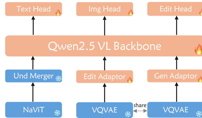
Stage 4: Unified Fine-tuning
