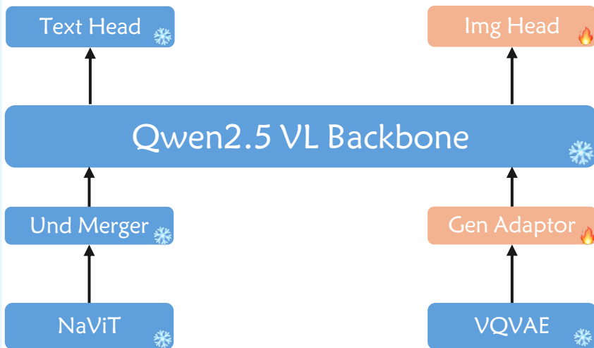
Stage 1: Preliminary Generation Alignment
