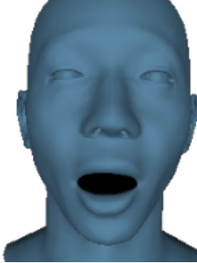
\rho = 3.0
