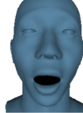
\rho = 4.0
