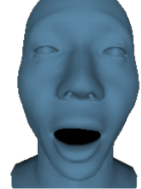
\rho = 5.0
