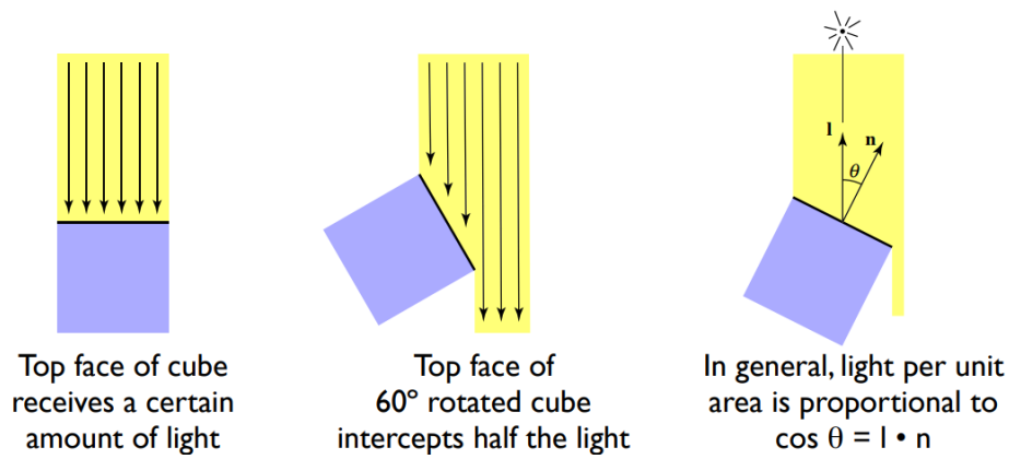
Figure 5.15: Lambert's Cosine Law
