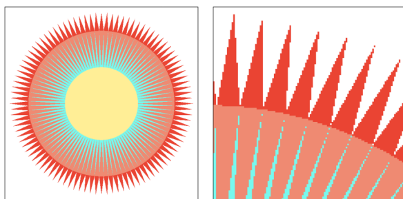
Figure 5.10: Point Sampling
