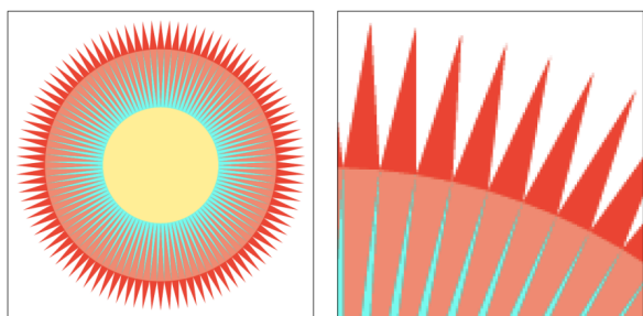
Figure 5.11: 4 \times 4 Supersampling
