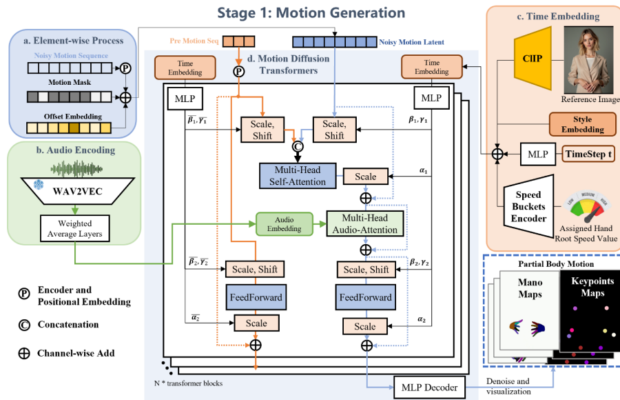
Figure 2. Overview of the stage 1 hand motion generation framework. The framework includes several DiT blocks as backbone. Audio embeddings are injected via cross-attention, style and speed embeddings are added on timestep, previous motion latent sequence is concatenated on current noisy motion latent sequence for smooth transition. Hand masks that mask out invisible hands frames are directly added on noisy motion latent.
