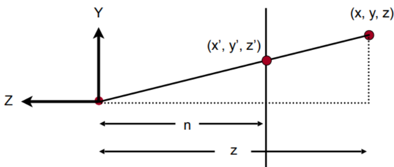
Figure 3.11: 透视投影变换为正交投影
