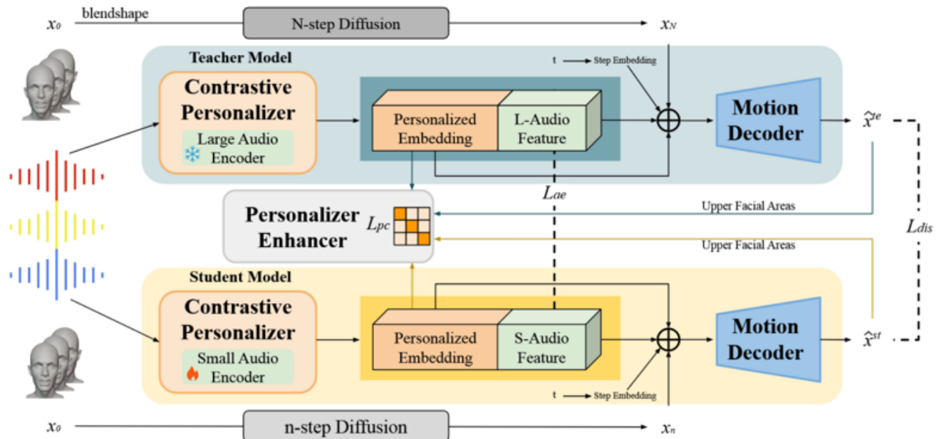
Figure 3.13: DiffusionTalker
