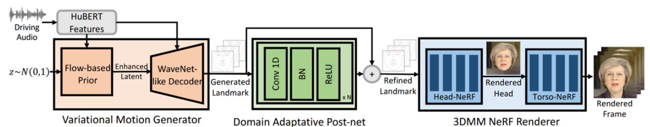
Figure 3.7: GeneFace
