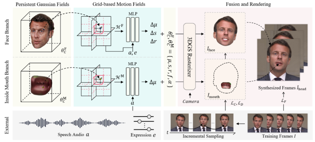
Figure 3.17: TalkingGaussian
