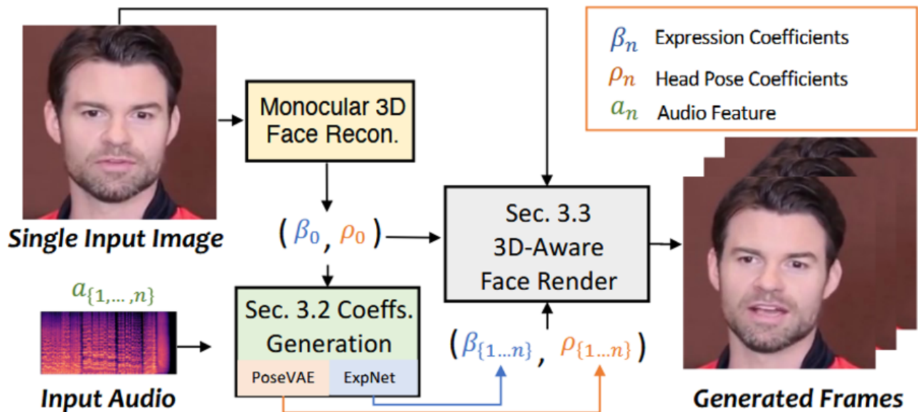
Figure 3.10: SadTalker
