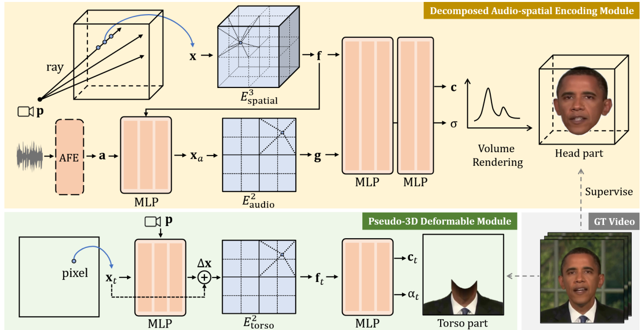
Figure 3.16: RAD-NeRF
