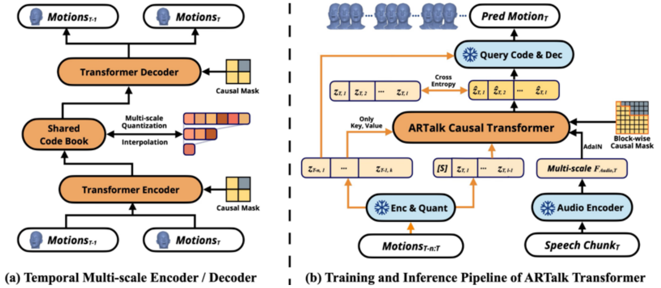
Figure 3.12: ARTalk
