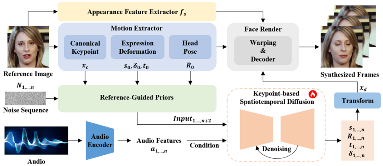
Figure 3.8: KDTalker
