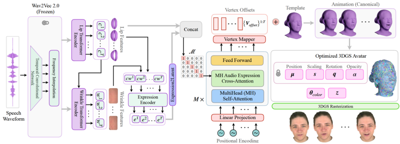
Figure 3.5: GaussianSpeech
