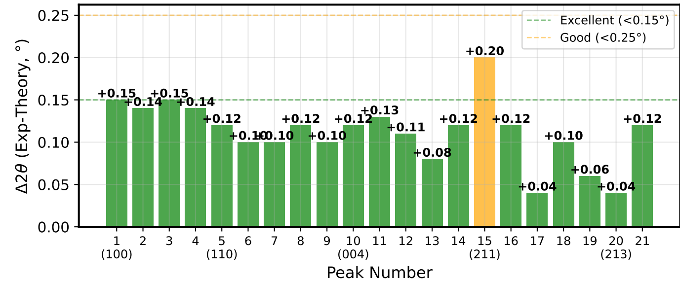
Peak Position Deviation for All 21 Peaks
