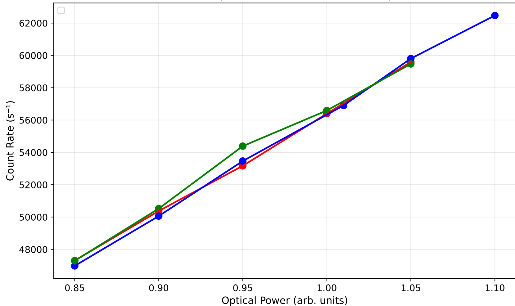
Count Rate vs Optical Power at Different Temperatures
