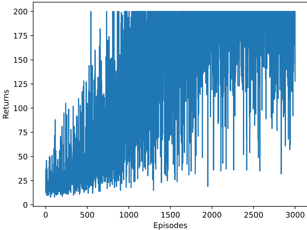
CartPole-v0
