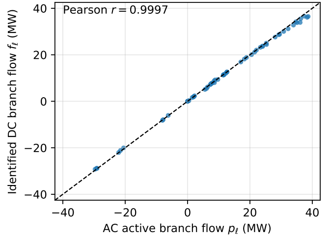
Fig. 1. Identified DC branch flows versus AC branch flows on rte_case14_realistic (three states, 60 branch observations). The identified model reproduces AC flows with Pearson correlation r = 0.9997 .
