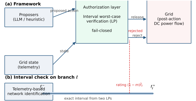
Fig. 2. Framework: proposers submit actions, the authorization layer releases them only if the exact worst case of the post-action branch-flow interval over the load uncertainty box satisfies the rating constraint (fail-closed on any numerical failure). The network model is identified from telemetry.
