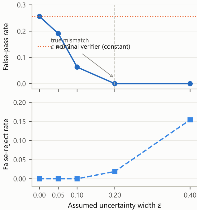
Fig. 7. False-pass and false-reject rates of the interval layer versus assumed uncertainty width \varepsilon (true mismatch fixed at 0.2). The false-pass rate is zero whenever \varepsilon covers the true mismatch.
