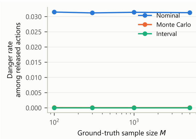
Fig. 4. Danger rate among released actions as a function of the ground-truth sample size M (nominal, Monte Carlo, and interval verifiers). The interval rate is identically zero; the nominal estimate stabilizes from M = 100 onward.
