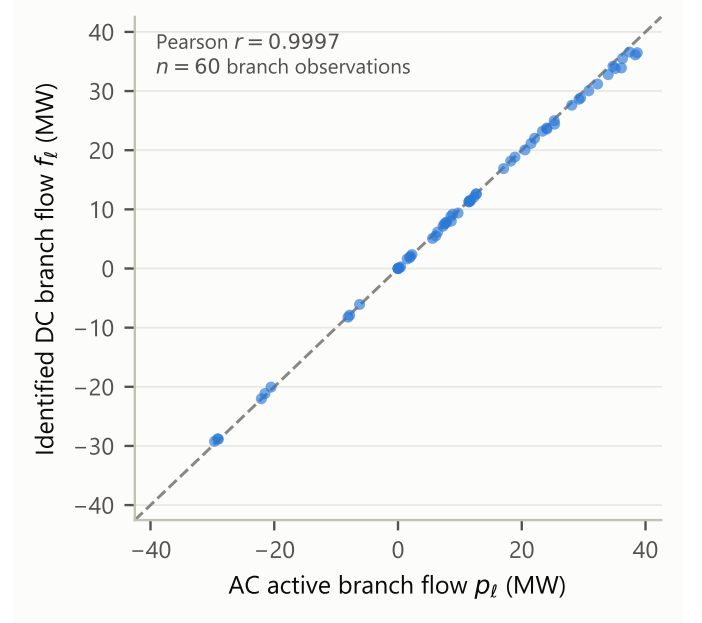
Fig. 1. Identified DC branch flows versus AC branch flows on rte_case14_realistic (three states, 60 branch observations). The identified model reproduces AC flows with Pearson correlation r = 0.9997 .
