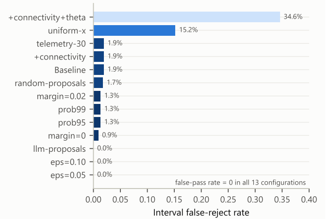
Fig. 6. False-reject rate of the interval layer across 13 ablation configurations; the false-pass rate is zero in every configuration.
