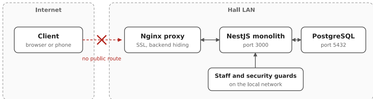
Figure 1. v0: LAN-only deployment, with no public route for Clients
