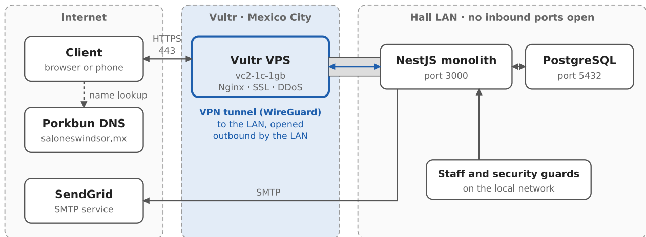
Figure 2. v1: public proxy on Vultr with a VPN tunnel to the hall LAN
