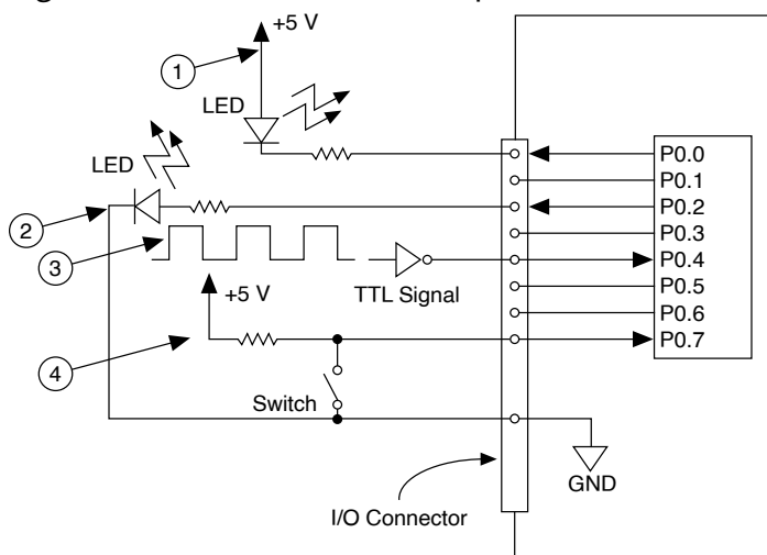
Figure 8. DIO Connections Example
