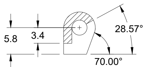
SECTION O-O
