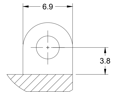
10 X DETAIL F SCALE 4:1
