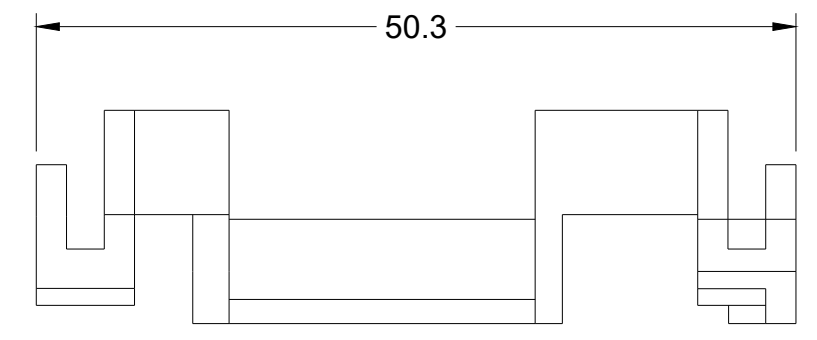
SECTION AE-AE
