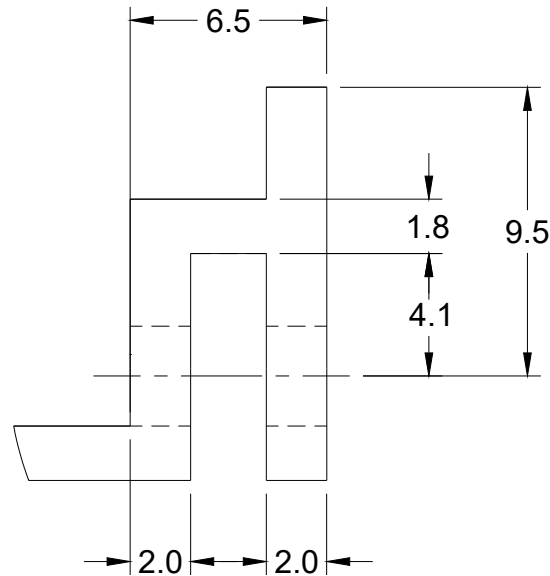
DETAIL R SCALE 4:1
