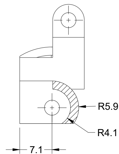
SECTION AD-AD
