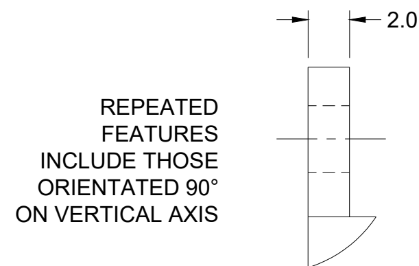
10 X DETAIL E SCALE 4:1
