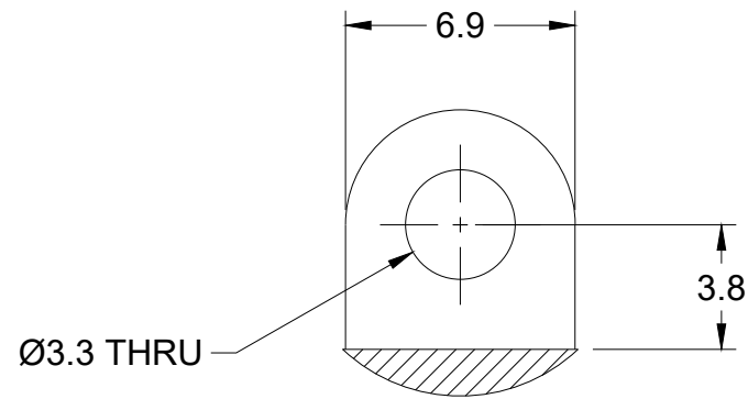
6 X DETAIL H SCALE 4:1
