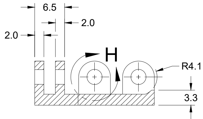
SECTION G-G
