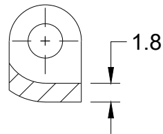
SECTION P-P
