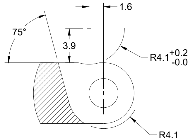
DETAIL AL SCALE 4:1
