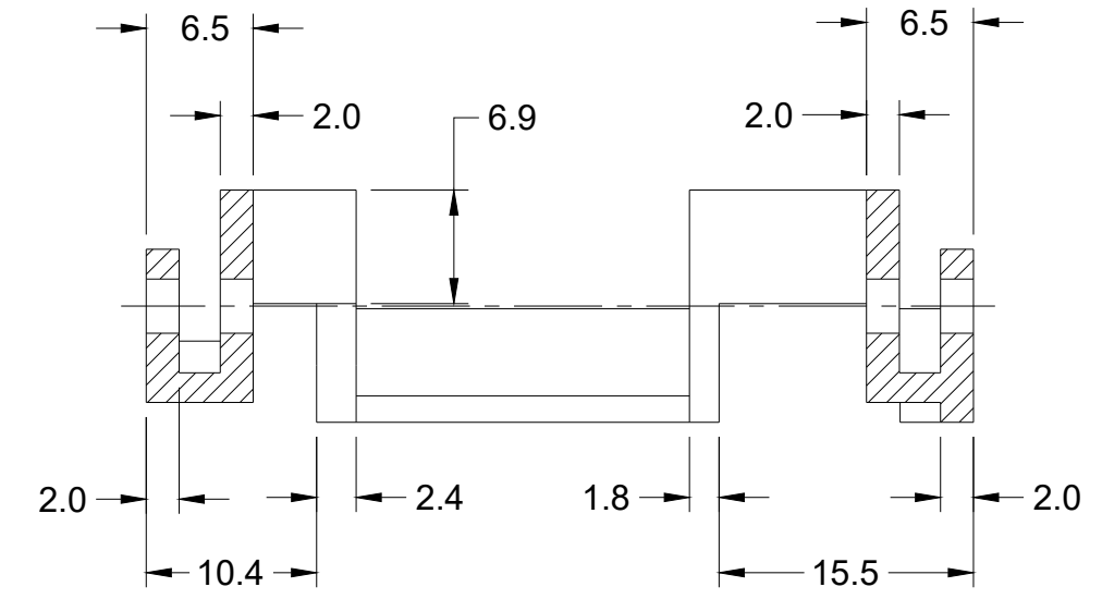
SECTION AE-AE
