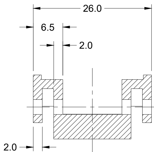
SECTION AH-AH
