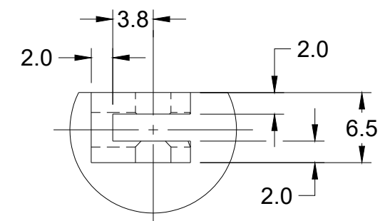
DETAIL D
