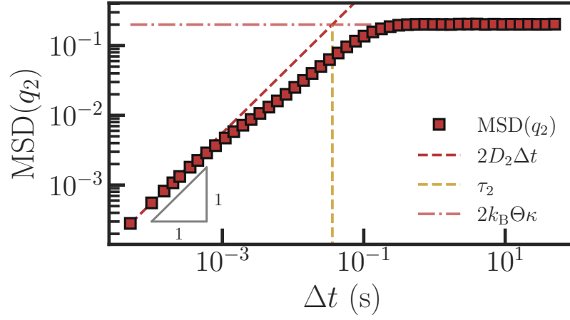
Figure 1.5: Mean-Squared Displacement of q_2 for \kappa = 0.01 , \Delta U = 2.7k_B\Theta , k_B\Theta = 1.0 , \lambda = 0.5 , \gamma_{11} = 1 , \gamma_{22} = 1 , \gamma_{12} = 0.8 , \tau = 10^{-4}\text{s} , for a single trajectory of N = 1 \times 10^8 points. At small timelags \Delta t < \tau_2 , the membrane presents a diffusion constant D_2 (Eq. 1.45, in red dashes) which corresponds to a bulk, free diffusivity inside the minimum of the harmonic potential. It then slowly crosses over to a second diffusive regime for \Delta t > \tau^2 with constant MSD. The dotted red line indicates the expected plateau value for the long-time MSD at 2k_B\Theta\kappa .
