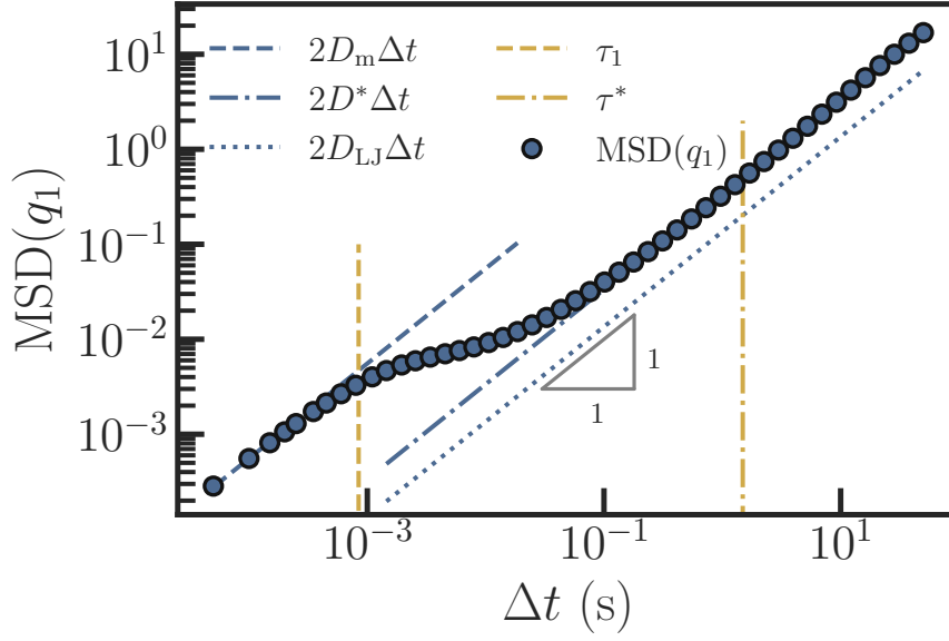
Figure 1.4: Mean-Squared Displacement of q_1 for \kappa = 0.01 , \Delta U = 2.7k_B\Theta , k_B\Theta = 1.0 , \lambda = 0.5 , \gamma_{11} = 1 , \gamma_{22} = 1 , \gamma_{12} = 0.8 , \tau = 10^{-4}\text{s} , for a single trajectory of N = 1 \times 10^8 points. At small timelags \Delta t < \tau_1 , the Brownian colloid presents a diffusion constant D_m (Eq. 1.44, in blue dashes) which corresponds to a bulk, free diffusivity inside a local minimum of the potential \phi(q_1) . It then slowly crosses over to a second diffusive regime for \Delta t > \tau^* with diffusion constant D^* (Eq. 1.30, in blue dashdot). The dotted blue line indicates the expected long-time diffusion coefficient in the very rigid limit \kappa \rightarrow 0 (Eq. 1.27 for \kappa = 0 ), which is smaller, as expected.
