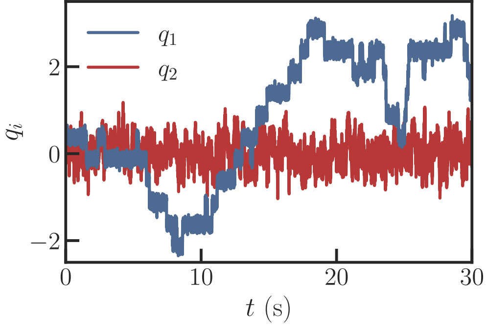
Figure 1.2: Trajectories of the Brownian colloid (blue) and the membrane (red) for \kappa = 0.01 . The other parameters are fixed to \Delta U = 2.7k_B\Theta , k_B\Theta = 1.0 , \lambda = 1.0 , \gamma_{11} = 1.0 , \gamma_{22} = 1.0 and \gamma_{12} = 0.8 , \tau = 10^{-4} . The membrane noticeably fluctuates around its equilibrium position in q_2 = 0 , whereas the colloid is trapped at short times within a local minimum, and escapes through random thermal fluctuations at longer times to explore available space.
