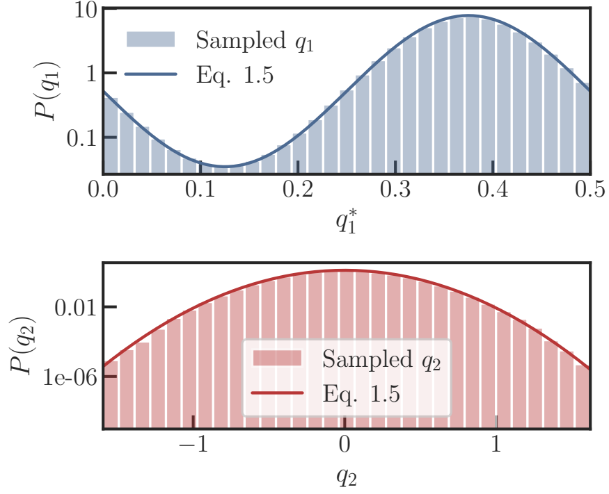
Figure 1.3: Equilibrium probability density function of q_1 (top, for q_1^* = q_1 \bmod \lambda ) and q_2 (bottom) for \kappa = 0.01 . The other parameters are fixed to \Delta U = 2.7k_B\Theta , k_B\Theta = 1.0 , \lambda = 1.0 , \gamma_{11} = 1 , \gamma_{22} = 1 , \gamma_{12} = 0.8 , \tau = 10^{-4}\text{s} , for a single trajectory of N = 1 \times 10^7 points. The sampled probability density functions (histograms) and theoretical prediction from the Gibbs-Boltzmann distribution (Eq. 1.5, solid lines) are in perfect agreement, even for a single trajectory of 10^8 points.
