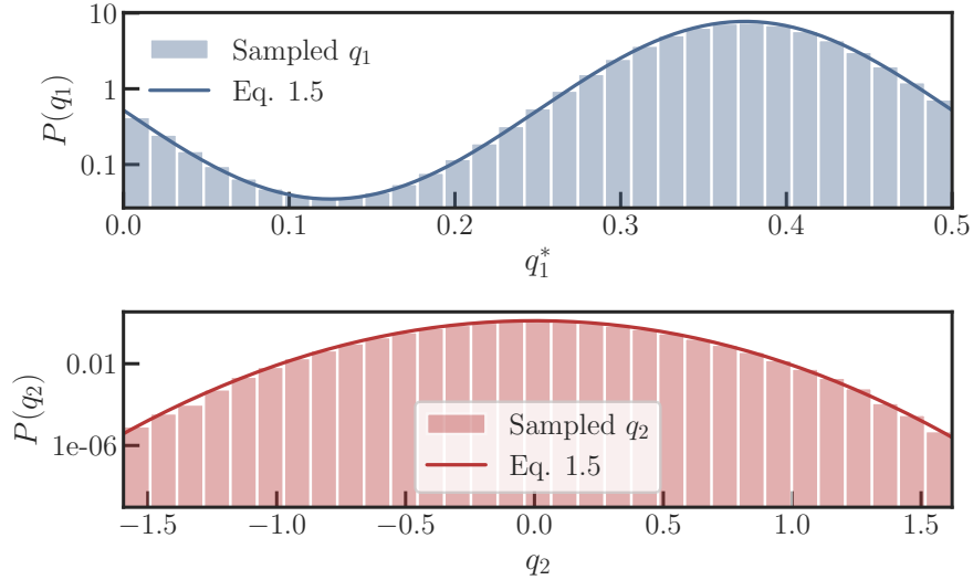
Figure 3.3: Equilibrium probability density function of q_1 (top, for q_1^* = q_1 \bmod \lambda ) and q_2 (bottom) for \kappa = 0.010 . The other parameters are fixed to \Delta U = 2.7k_B\Theta , k_B\Theta = 1.0 , \lambda = 1.0 , \gamma_{11} = 1.0 , \gamma_{22} = 1.0 , \gamma_{12} = 0.8 , \tau = 10^{-4} s, for a single trajectory of N = 1.0 \times 10^7 points. The sampled probability density functions (histograms) and theoretical prediction from the Gibbs-Boltzmann distribution (Eq. 3.5, solid lines) are in perfect agreement, even for a single trajectory of 10^8 points.
