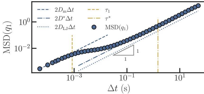
Figure 3.4: Mean-Squared Displacement of q_1 for \kappa = 0.01 , \Delta U = 2.7k_B\Theta , k_B\Theta = 1.0 , \lambda = 0.5 , \gamma_{11} = 1 , \gamma_{22} = 1 , \gamma_{12} = 0.8 , \tau = 10^{-4}\text{s} , for a single trajectory of N = 1 \times 10^8 points. At small timelags \Delta t < \tau_1 , the Brownian colloid presents a diffusion constant D_m (Eq. 3.44, in blue dashes) which corresponds to a bulk, free diffusivity inside a local minimum of the potential \phi(q_1) . It then slowly crosses over to a second diffusive regime for \Delta t > \tau^* with diffusion constant D^* (Eq. 3.30, in blue dashdot). The dotted blue line indicates the expected long-time diffusion coefficient in the very rigid limit \kappa \rightarrow 0 (Eq. 3.27 for \kappa = 0 ), which is smaller, as expected.
