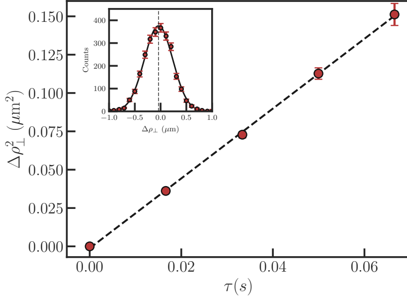
Figure 2.7: Adapted from [7]. Measured pair diffusion for the relative perpendicular mode of motion of the two colloids. The upper inset shows the histogram of all binned displacements for a given time step, for h = 25.5 \pm 0.7 \mu\text{m} and r = 7.00 \pm 0.25 \mu\text{m} . This process is repeated over all time steps and each histogram is fitted with a Gaussian curve to recover the root mean square displacement \Delta\rho(r, h, \tau) to recover the MSD of the main plot. The effective cross-diffusion coefficient for the perpendicular mode is then extracted from the slope of the MSD.
