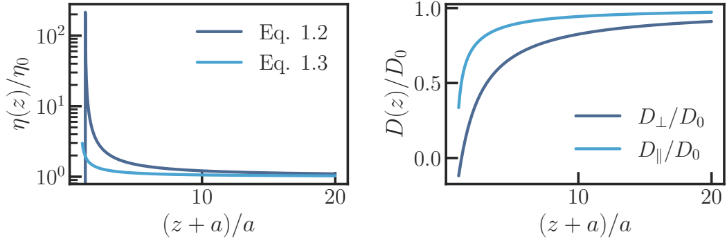
Figure 2.3: Effective viscosities and corresponding effective diffusion coefficients for a colloid diffusing over a plane. Left panel: Effective viscosities \eta_\perp (navy) and \eta_\parallel (sky blue) renormalised by the bulk viscosity \eta_0 as a function of the distance to the wall z . Right panel: Effective diffusion coefficients D_\perp (navy) and D_\parallel (sky blue) renormalised by the bulk diffusion coefficient D_0 as a function of the renormalised colloid center-to-wall distance (z+a)/a .
