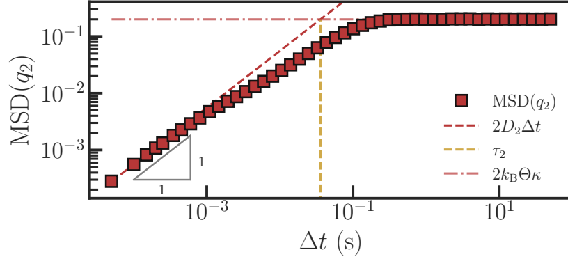
Figure 3.5: Mean-Squared Displacement of q_2 for \kappa = 0.01 , \Delta U = 2.7k_B\Theta , k_B\Theta = 1.0 , \lambda = 0.5 , \gamma_{11} = 1 , \gamma_{22} = 1 , \gamma_{12} = 0.8 , \tau = 10^{-4}\text{s} , for a single trajectory of N = 1 \times 10^8 points. At small timelags \Delta t < \tau_2 , the membrane presents a diffusion constant D_2 (Eq. 3.45, in red dashes) which corresponds to a bulk, free diffusivity inside the minimum of the harmonic potential. It then slowly crosses over to a second diffusive regime for \Delta t > \tau^2 with constant MSD. The dotted red line indicates the expected plateau value for the long-time MSD at 2k_B\Theta\kappa .
