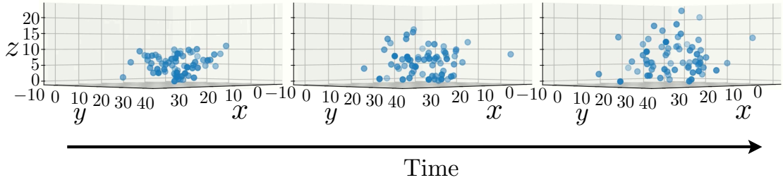
Figure 4.8: Numerical simulation results at initialisation and through time, for a bad initialisation of the system. Colloids were laced in a 10\text{ }\mu\text{m} tall box and left to thermalise with l_B = 1.1 \times 10^{-2}\text{ m} . As expected, colloids escape the boundaries of the original box from thermal fluctuations, thus effectively reducing the volume fraction inside the box.
