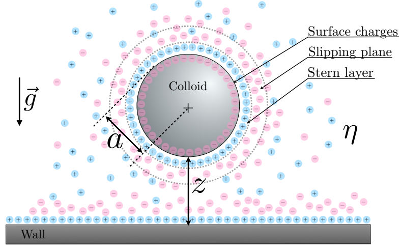
Figure 2.4: Schematic representation of a colloid of radius a at a distance z from an infinite plane. Both surfaces are charged, and thus, a double layer of counter-ions forms around each of them.
