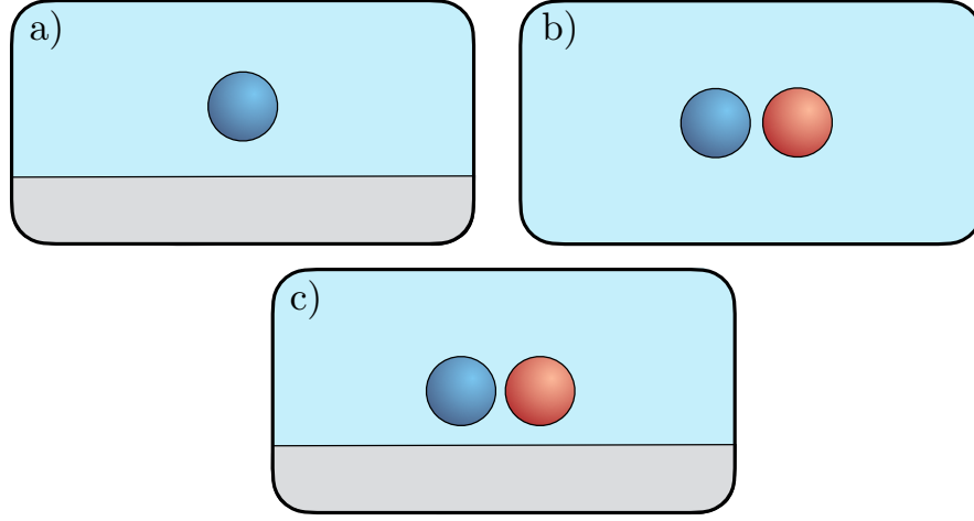
Figure 2.1: Schematic representation of the three cases of interest for this Chapter. a) A single colloid diffusing in a fluid over an infinite, hard boundary. b) Two colloids interacting with each other through hydrodynamic interactions in an unbounded fluid. c) A combination of the two first cases, where two colloids interact with each other and with an infinite, hard boundary.
