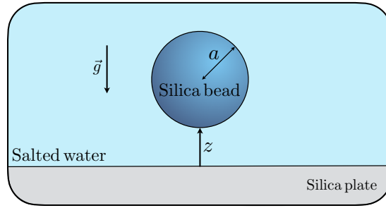
Figure 2.2: Schematic representation of a colloid of radius a at a distance z from an infinite plane.
