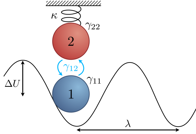
Figure 3.1: Representation of the system. A Brownian colloid of interest (blue) is trapped in a periodic potential of amplitude \Delta U and spatial period \lambda . An elastic membrane is modelled locally as a second Brownian colloid (red) subject to a harmonic potential of inverse stiffness (or compliance ) \kappa . This membrane is coupled to the colloid of interest through an indirect, hydrodynamic-like coupling represented by the coefficient \gamma_{12} , and both the colloid and the membrane feel their own self-friction \gamma_{11} and \gamma_{22} , respectively.
