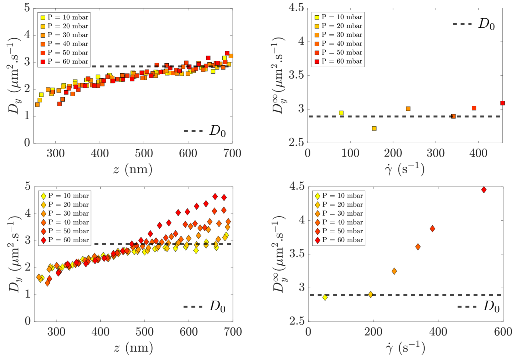
Figure 4.6: Transverse diffusion coefficients computed for \phi = 5.4 \times 10^{-6} (top) and \phi = 3.7 \times 10^{-5} (bottom) and for various pressure gradients \Delta P or equivalent shear rates \dot{\gamma} (in colours). Left panels show the diffusion at binned heights z above the channel wall. We notice a strong dependence of D_y on z in both cases, with a drop in diffusion as the colloid diffuses closer to the wall, which is to be expected from Brenner and Faxen's laws. However, once the colloid moves away from the wall, D_y picks up and may even reach higher values than the bulk value D_0 = 3.9 \mu\text{m}^2 \cdot \text{s}^{-1} (in horizontal dashed lines). This effect seems even more noticeable with higher \dot{\gamma} , as shown on the bottom right panel, where D_y^\infty indicates the diffusion coefficient very far from wall interactions. Adapted from [56].
