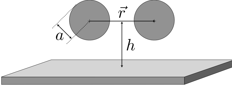
Figure 1.2: Experimental setup of Dufresne et al. [6] for the study of two colloids diffusing over a plane wall.
