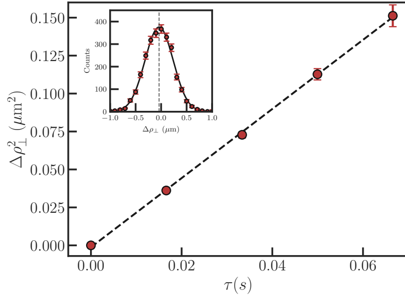
Figure 1.3: Adapted from [6]. Measured pair diffusion for the relative perpendicular mode of motion of the two colloids. The upper inset shows the histogram of all binned displacements for a given time step, for h = 25.5 \pm 0.7 \mu\text{m} and r = 7.00 \pm 0.25 \mu\text{m} . This process is repeated over all time steps and each histogram is fitted with a Gaussian curve to recover the root mean square displacement \Delta\rho(r, h, \tau) to recover the MSD of the main plot. The effective cross-diffusion coefficient for the perpendicular mode is then extracted from the slope of the MSD.
