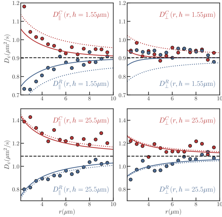
Figure 1.4: Adapted from [6]. Measured cross-diffusion coefficients for the relative perpendicular and parallel modes of motion of the two colloids, as a function of the center-to-center distance r between the colloids, for different values of the center-to-wall distance h . The dash lines correspond to the naive superposition of Oseen and Blake approximations, while the solid lines correspond to the more accurate approximation taking into account the interaction with the image colloid.
