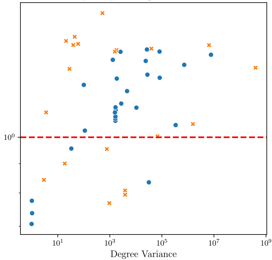
Speedup vs Degree Variance
