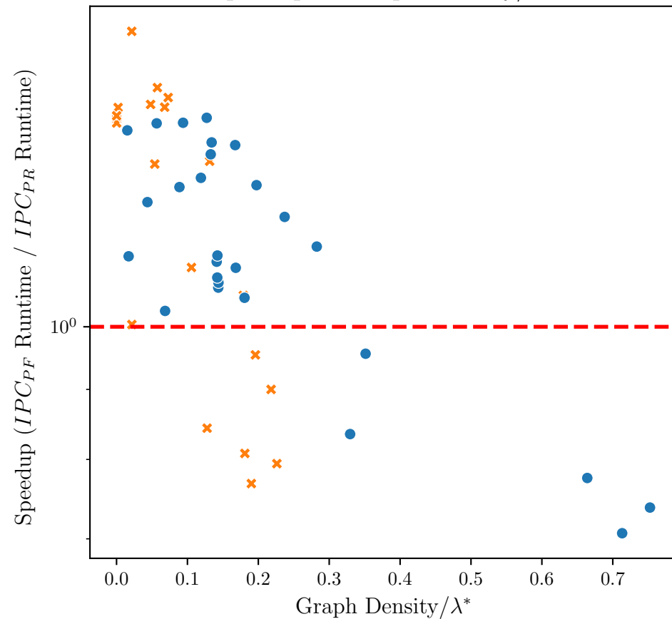
Speedup vs Graph Density/ \lambda^*
