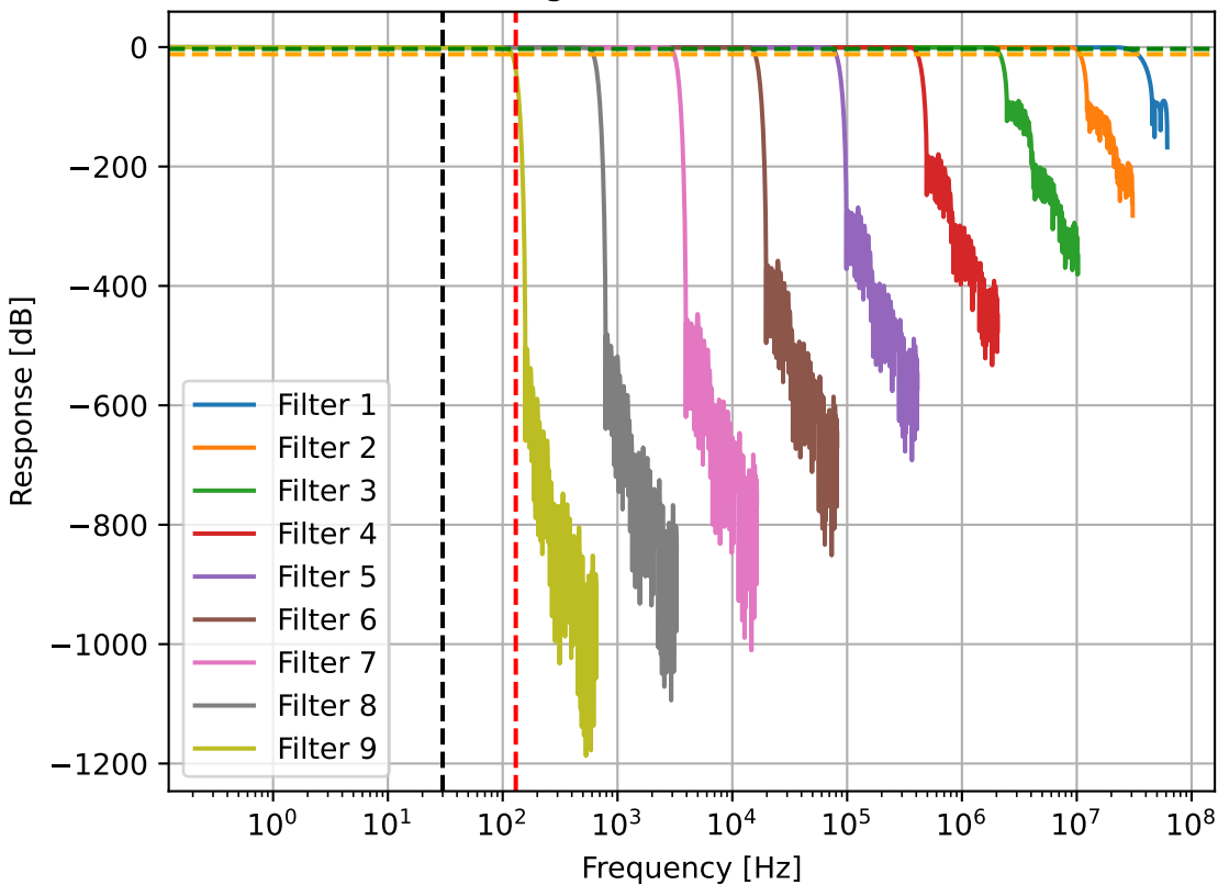
Filtering after downconversion
