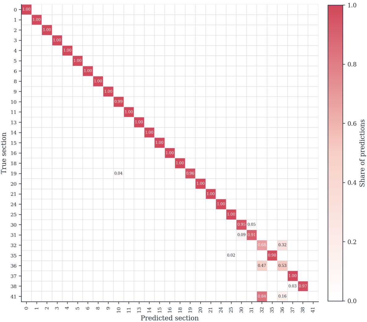
Figure 8. Confusion matrix for the supply subnet, excluding the "no defect" class.
