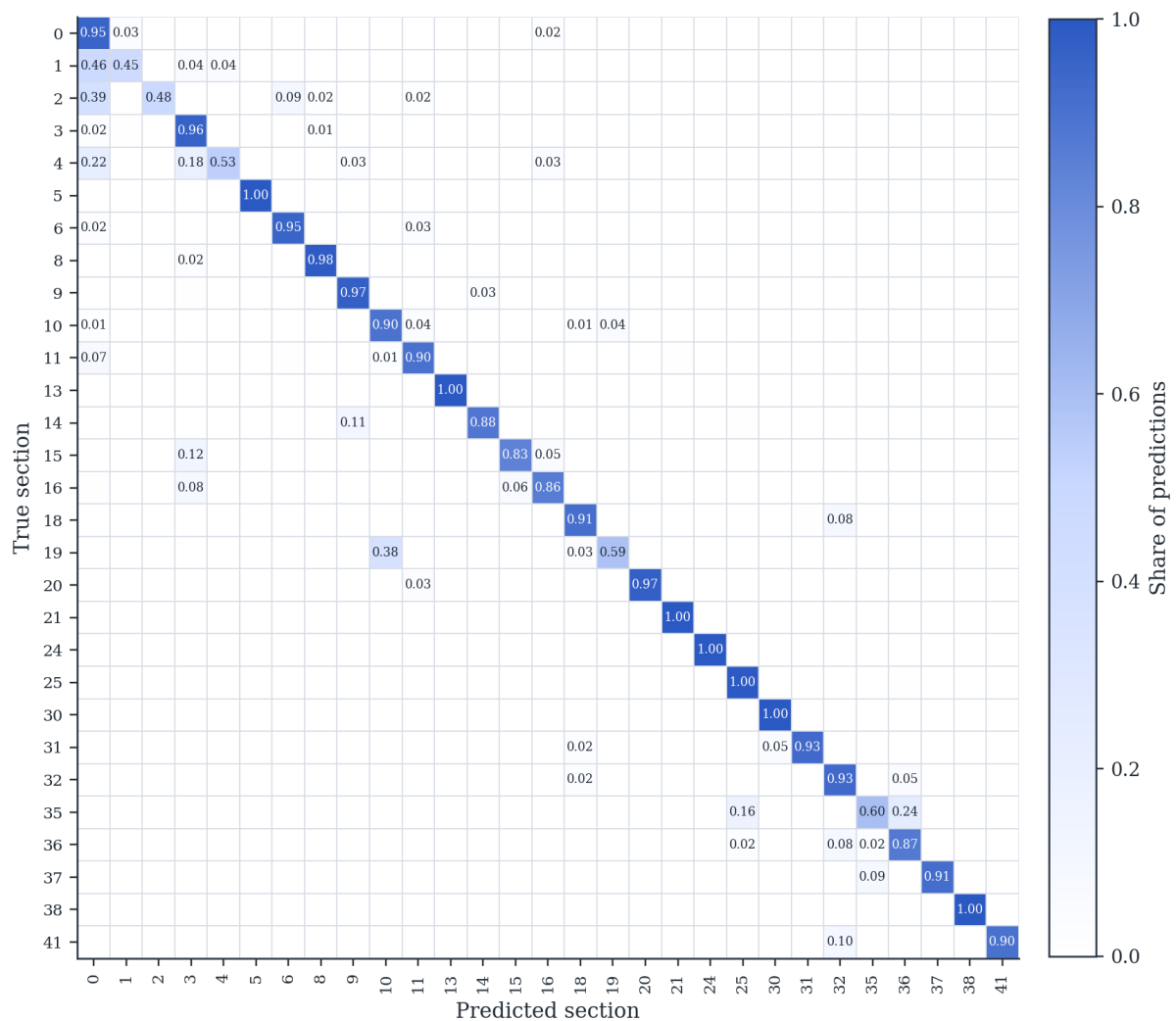
Figure 9. Confusion matrix for the return subnet, excluding the "no defect" class.
