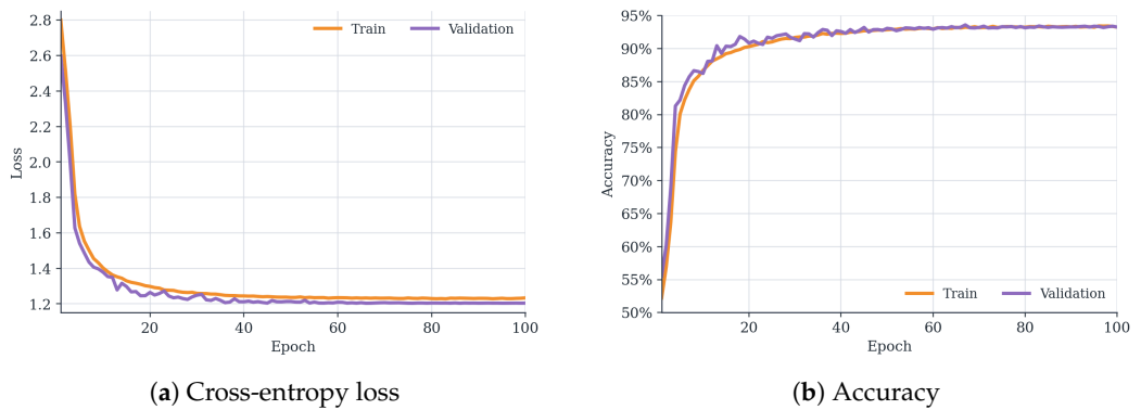
Figure 4. Training vs. validation performance over epochs.
