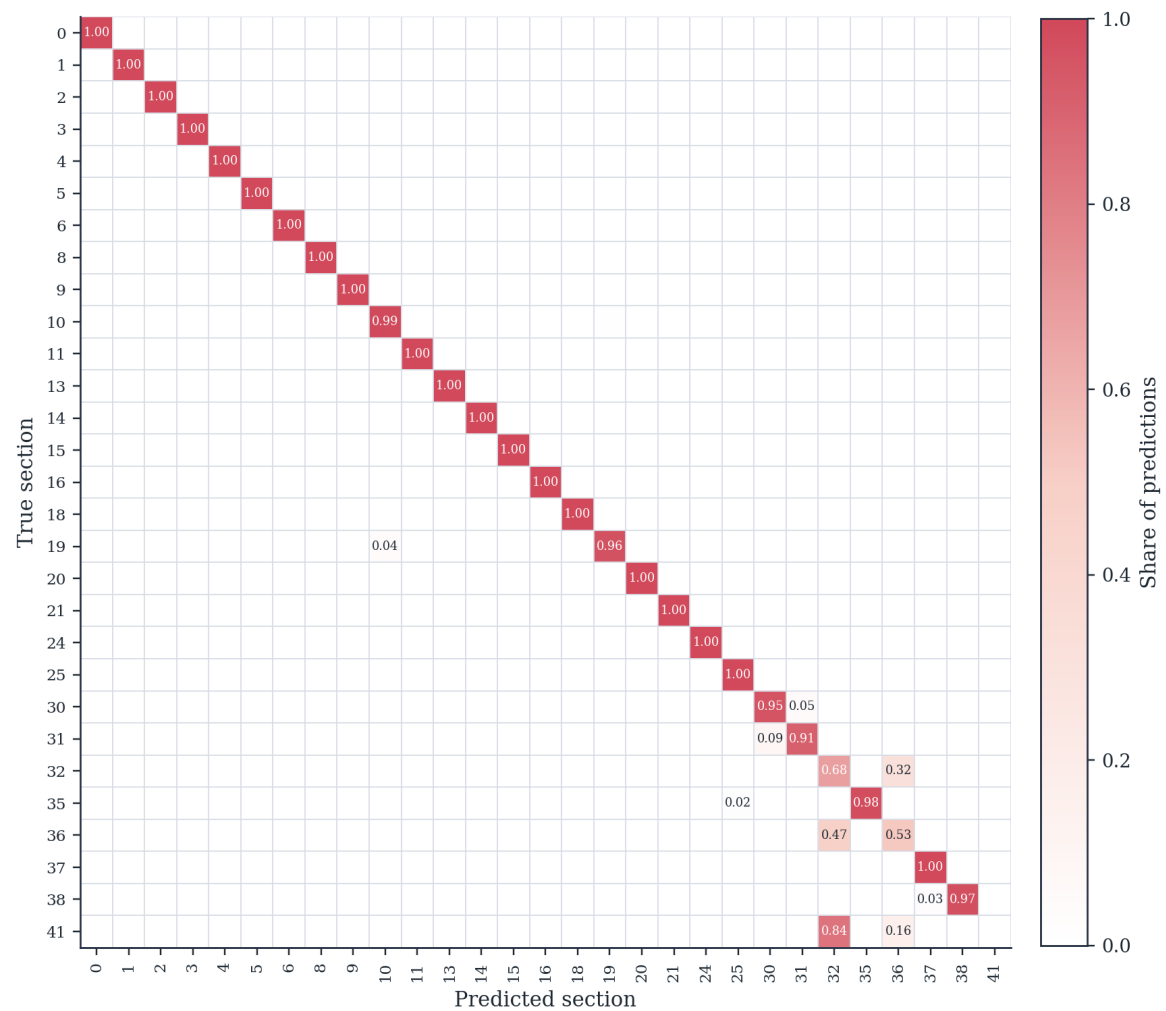
(b) Normalized confusion matrix
