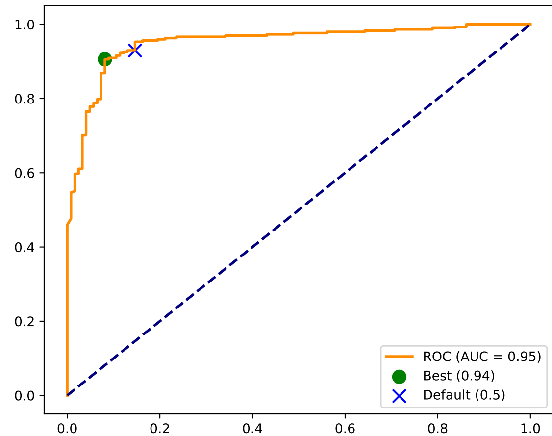
G-Mean Optimization
