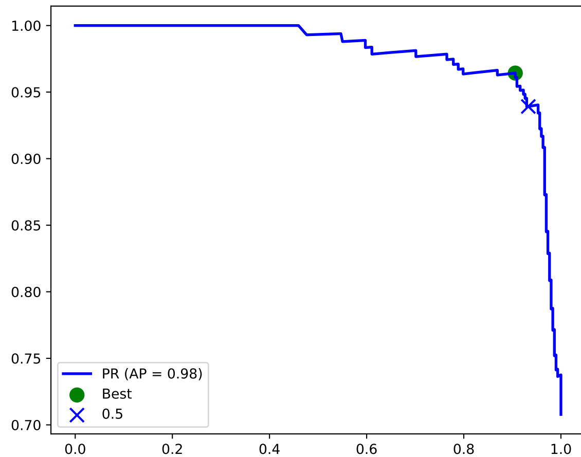
G-Mean Optimization
