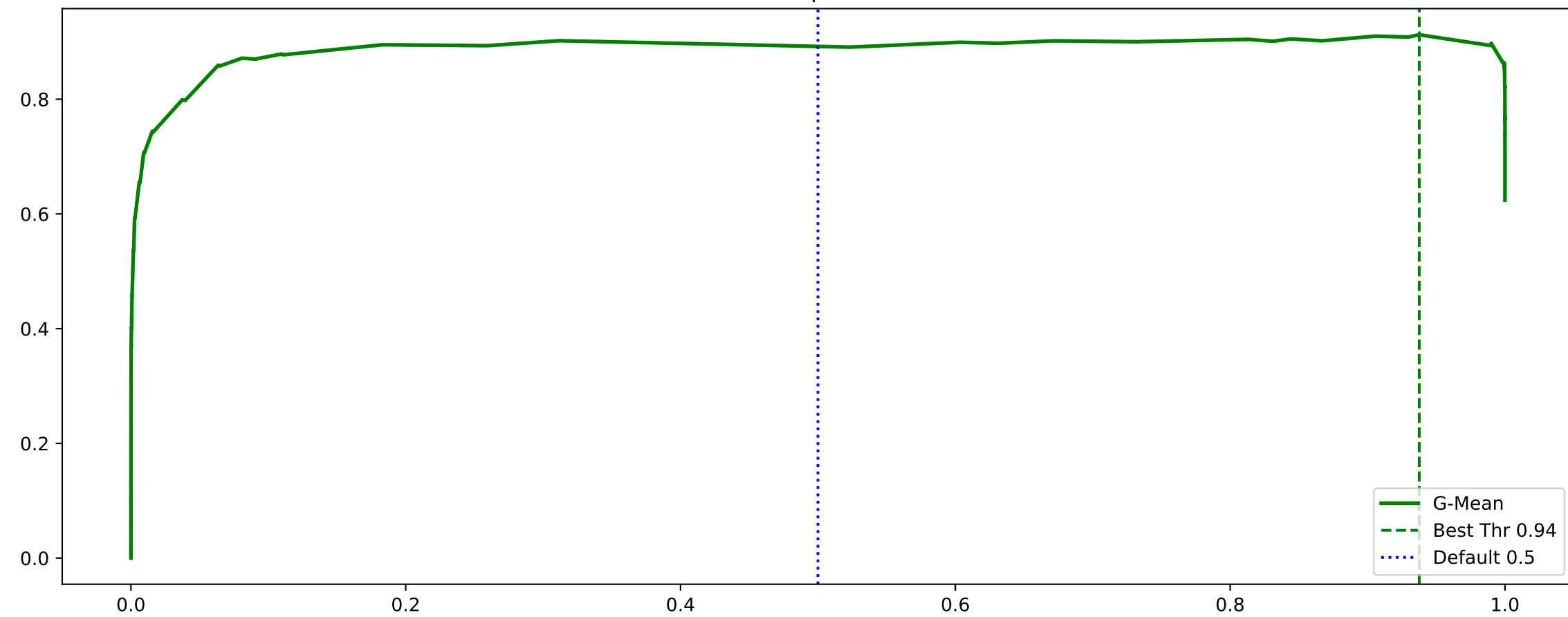
G-Mean Optimization
