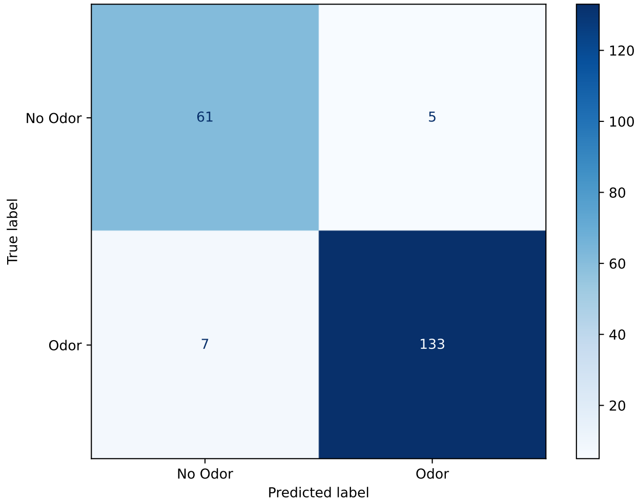
Confusion Matrix (Optimal Threshold 0.19)
