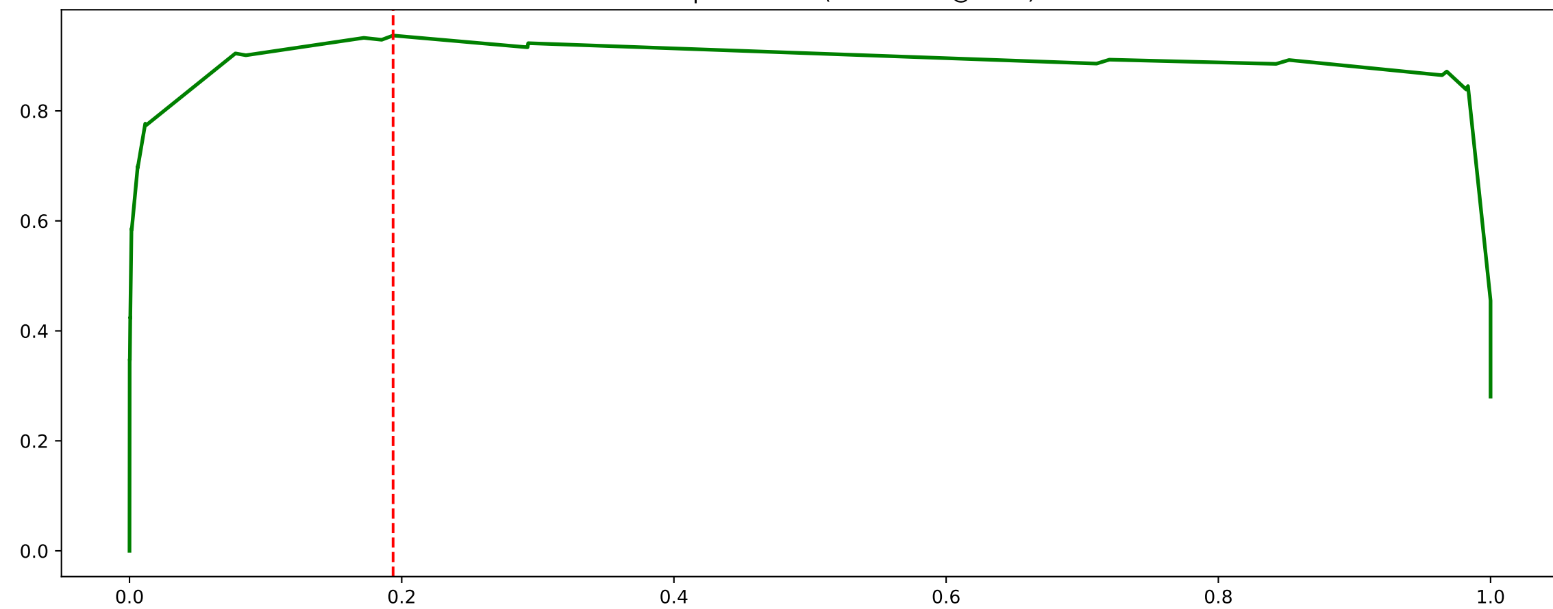
G-Mean Optimization (Best: 0.94 @ 0.19)
