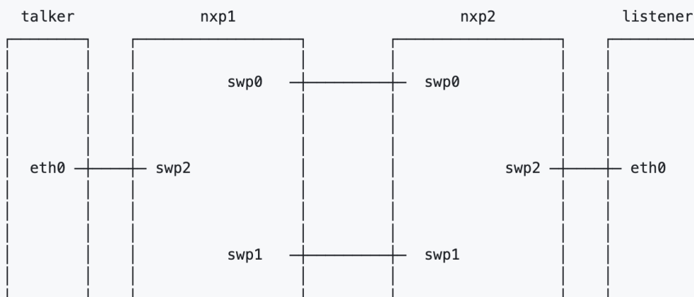
Fig 1: Scenario-1 topology
