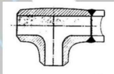
Gambar 2.7 Equal tee
