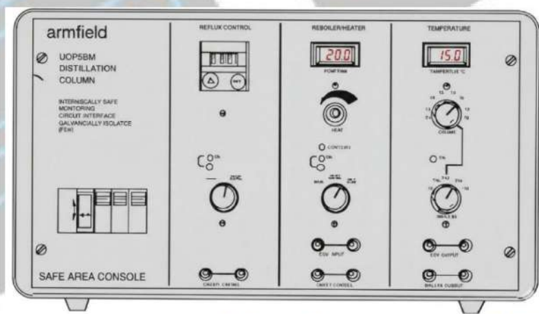
Gambar 3.4 Control panel alat distilasi batch
