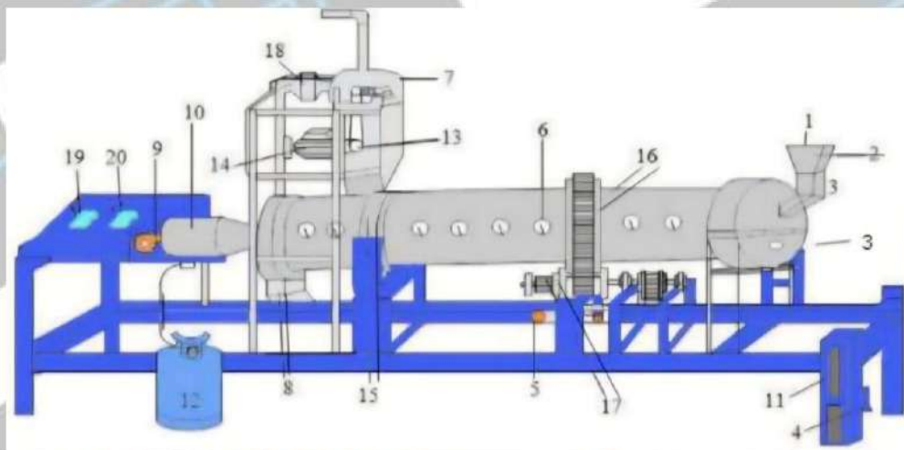
Gambar 3.1 Rotary dryer
