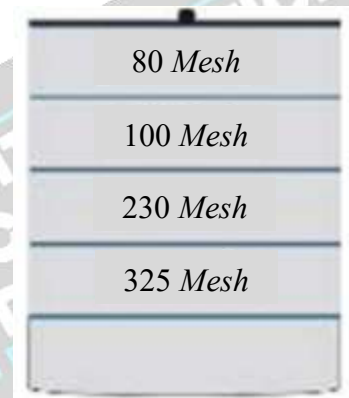
Gambar 3.3 Alat sieving (Shashidhar et al. , 2013)
