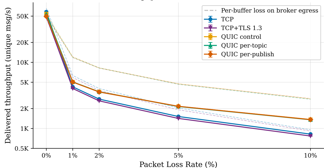
Delivered Throughput vs. Packet Loss Rate (QoS 0)
