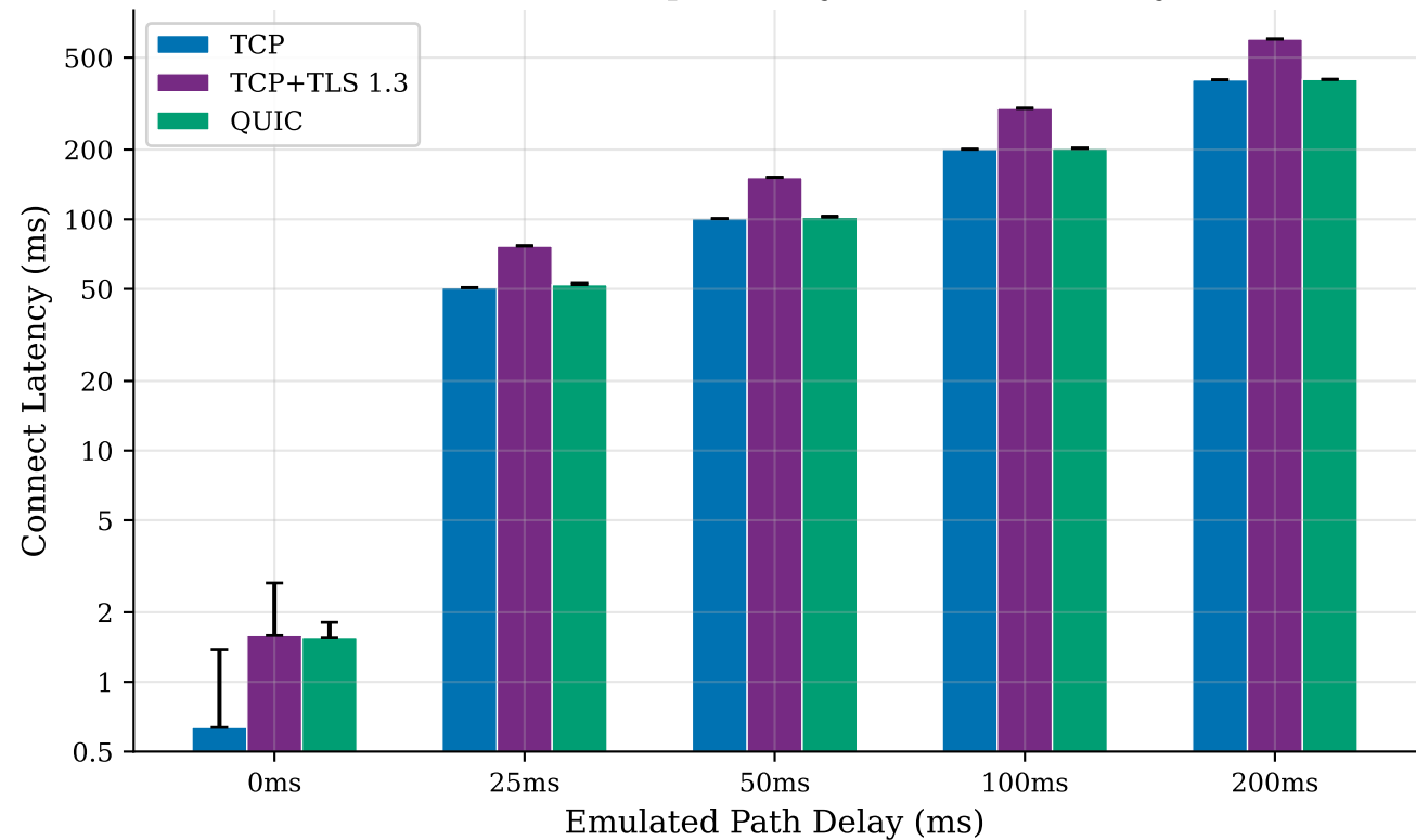
Connection Setup Latency vs. Network Delay
