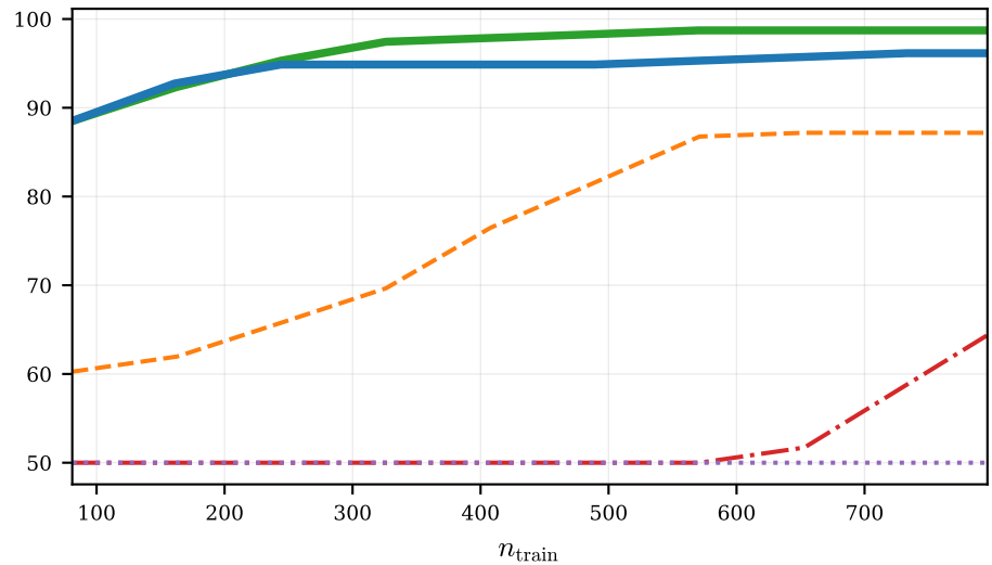
Tox21
