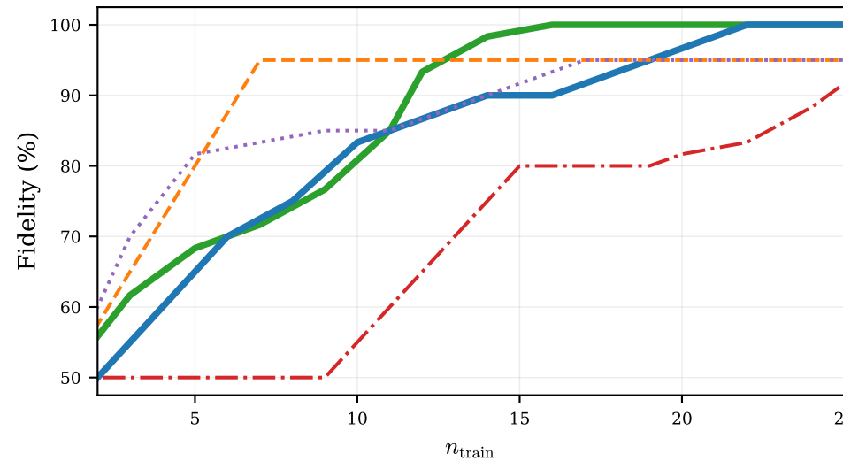
MUTAG
