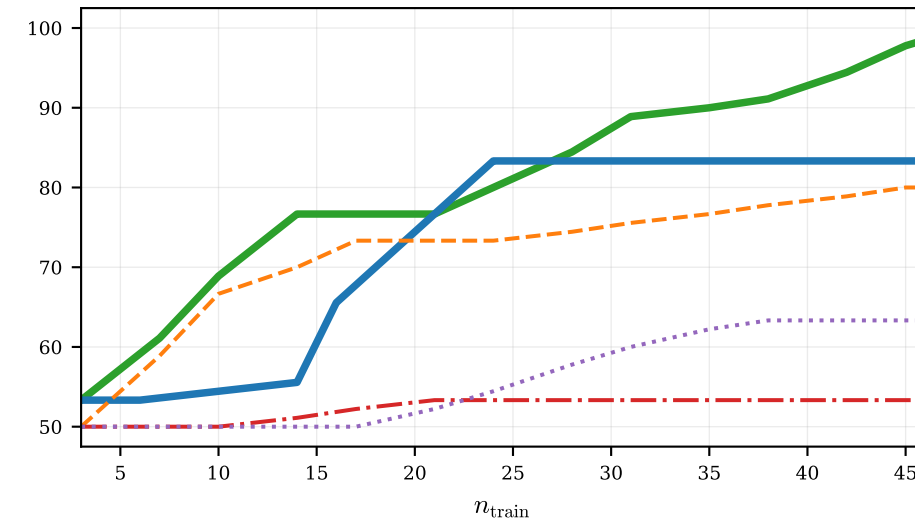
PTC_FM
