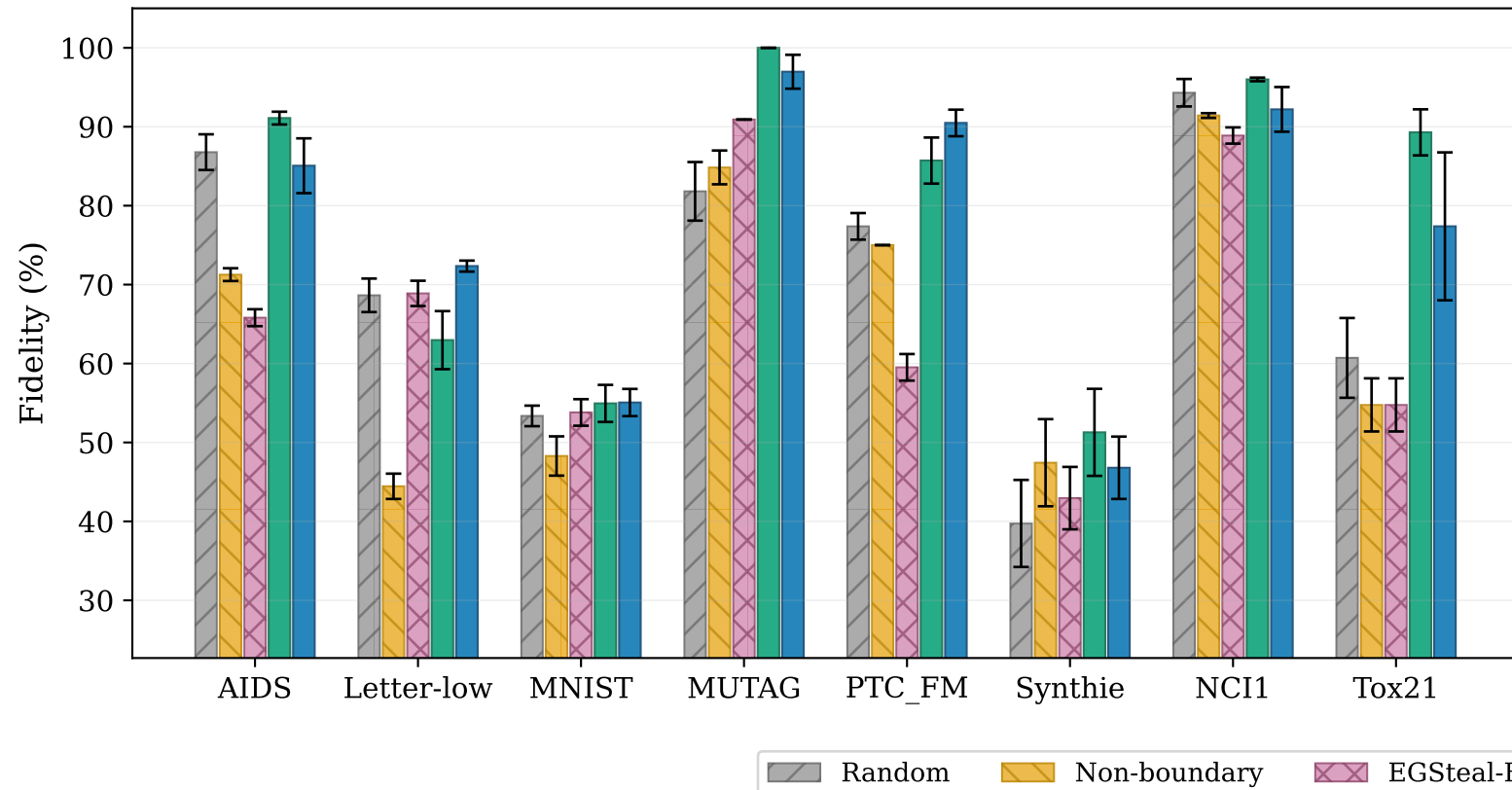
GNNExplainer
