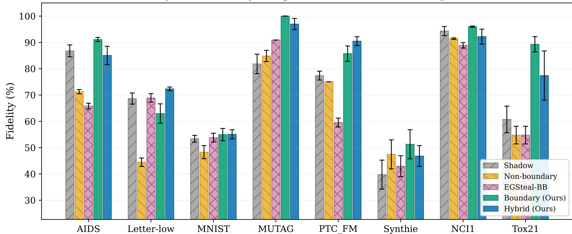
Fidelity at 70% Query Budget — GCN Victim (GNNExplainer)
