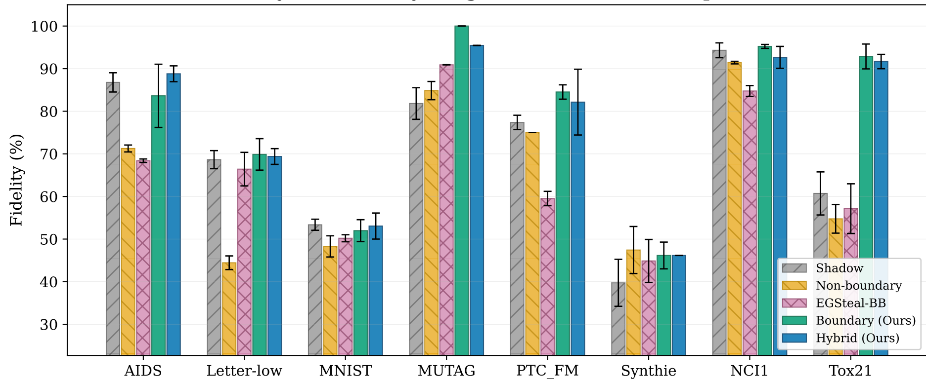
Fidelity at 70% Query Budget — GCN Victim (PGExplainer)
