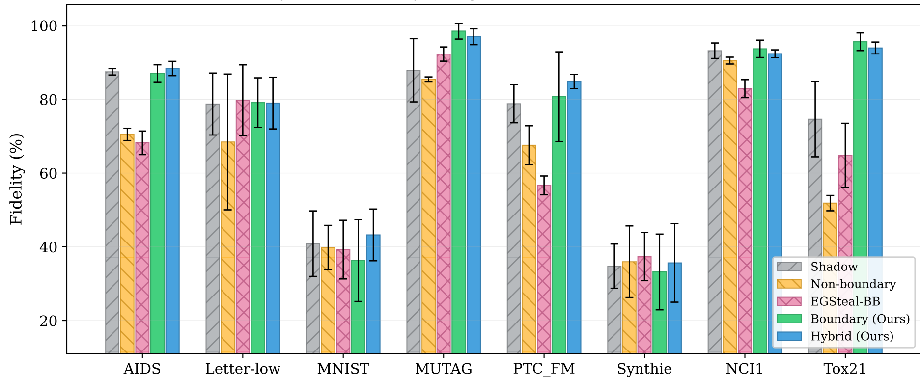
Fidelity at 70% Query Budget — All Victims (PGExplainer)
